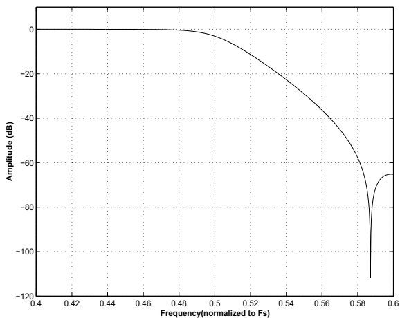
Figure 25. Single-Speed (slow) Transition Band
