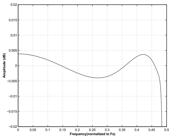
Figure 23. Single-Speed (fast) Passband Ripple
