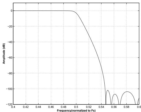
Figure 21. Single-Speed (fast) Transition Band
