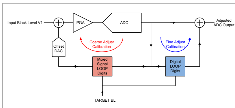
Figure 25 BLC Top-Level Circuitry
