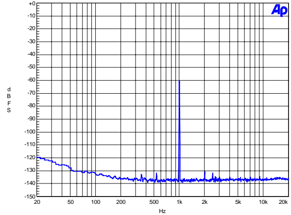
Figure 20. FFT (-60 dB, 96 kHz)
