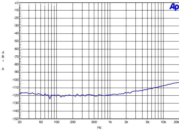
Figure 43. 48 kHz, Crosstalk
