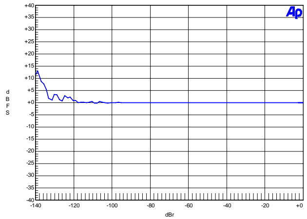
Figure 24. 96 kHz, Fade-to-Noise Linearity
