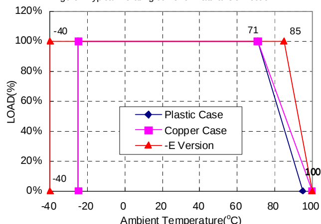
Figure1. Typical Derating curve for Natural Convection
