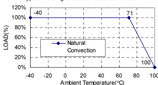
Typical Derating curve for Natural Convection
