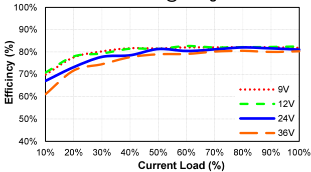
EC7AW-24S33 Eff Vs Io @25 Deg. C
