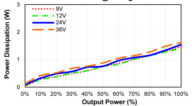
EC7AW-24S33 Pd Vs Po @25 Deg. C
