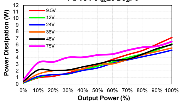
CQB50W8-36S24-CMFC Pd Vs Po @25 Deg. C
