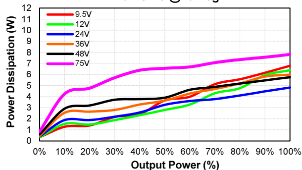
CQB50W8-36S48-CMFC Pd Vs Po @25 Deg. C
