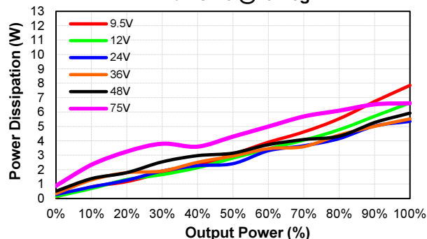
CQB50W8-36S15-CMFC Pd Vs Po @25 Deg. C
