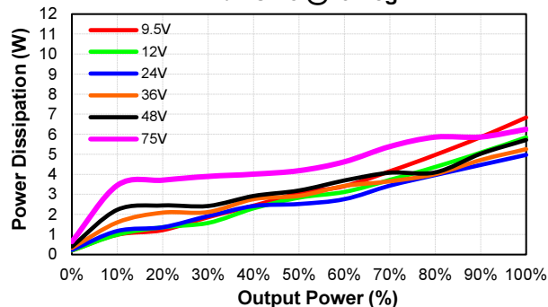
CQB50W8-36S28-CMFC Pd Vs Po @25 Deg. C
