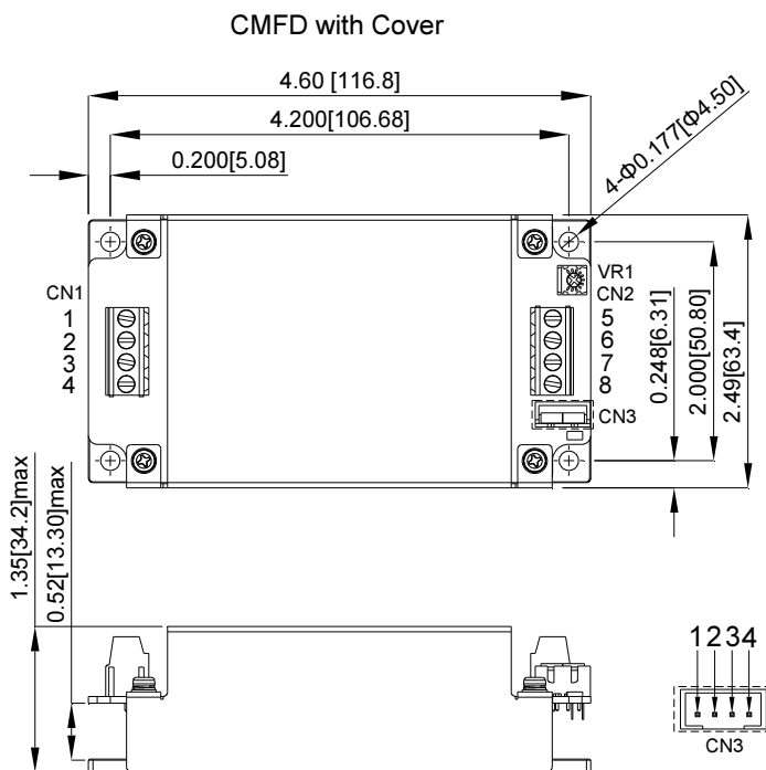
CN1&CN2 PIN CONNECTION
