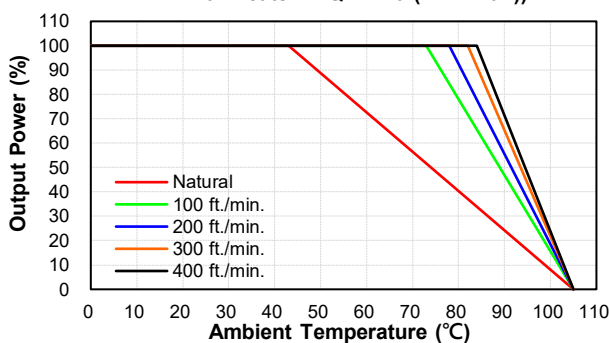
CQB150W-110S3V3,24,28 Derating Curve with Heatsink QBT210 (Vin=110V)
