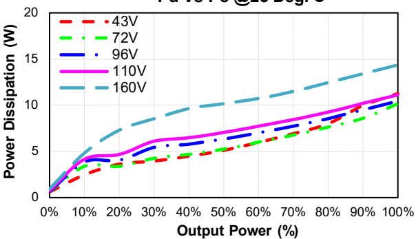
CQB100W-110S48-CMFC Pd Vs Po @25 Deg. C
