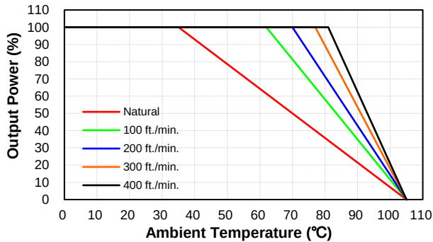
CHB150W-48S12 Derating Curve with Heatsink HBT127 (Vin=Nominal)
