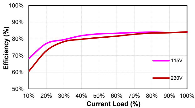
CFM60T-01 (Eff Vs Io)
