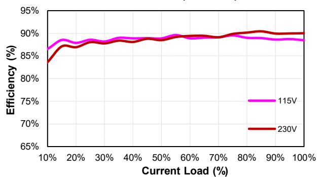
CFM60M480 (Eff Vs Io)
