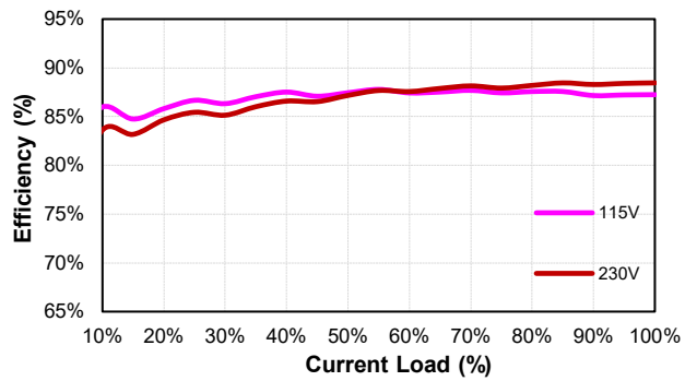
CFM60M150 (Eff Vs Io)
