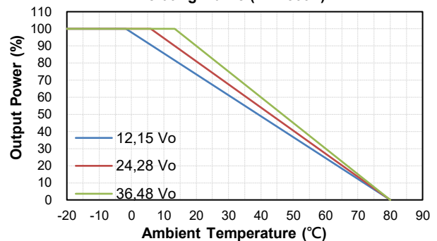
CFB750-300S CMFD+HS(HD) Derating Curve (Vin=300V)
