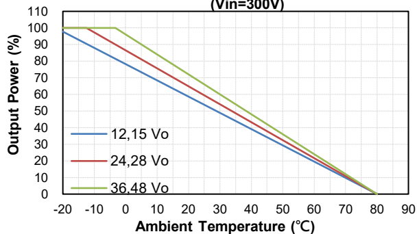
CFB750-300S CMFD Derating Curve with Aluminum Extrusion (9.84x4.33x1.57 inch) (Vin=300V)
