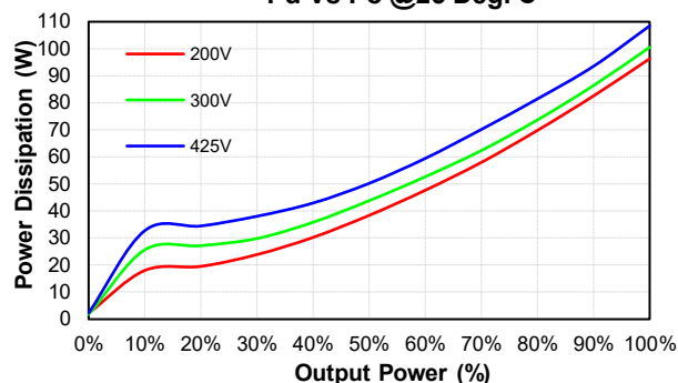
CFB750-300S12(N)-CMFD Pd Vs Po @25 Deg. C
