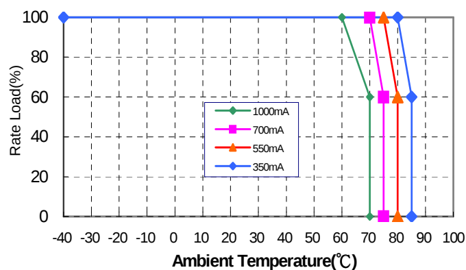
DIM01HXXW Derating Curve
