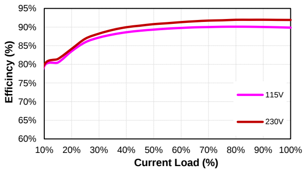
TR160M120 (Eff Vs Io)
