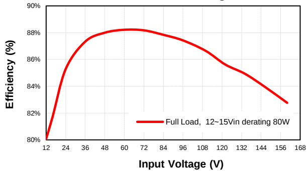
CQB100W14-72S05 Eff Vs Vin @25 Deg. C
