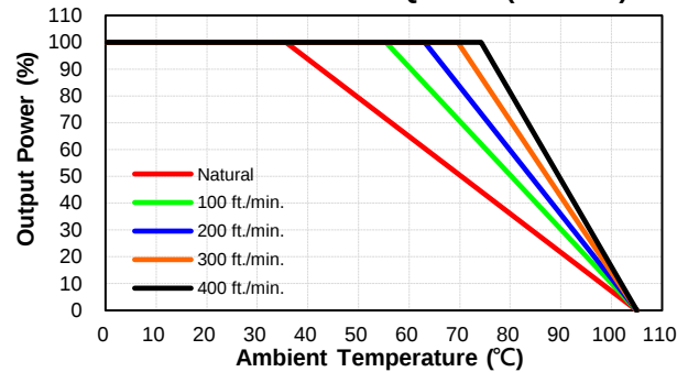
CQB100W14-72S15, 24, 28, 54 Derating Curve with Heatsink QBL127 (Vin=72V)
