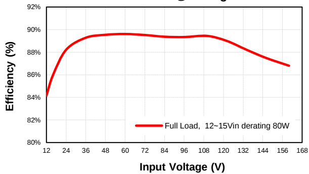
CQB100W14-72S15 Eff Vs Vin @25 Deg. C
