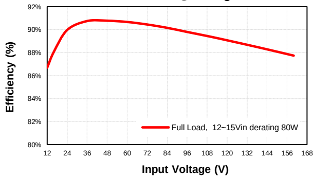
CQB100W14-72S28 Eff Vs Vin @25 Deg. C
