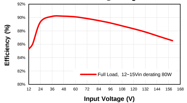
CQB100W14-72S24 Eff Vs Vin @25 Deg. C
