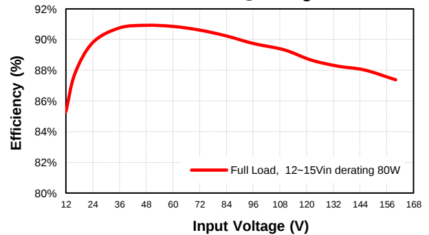
CQB100W14-72S54 Eff Vs Vin @25 Deg. C
