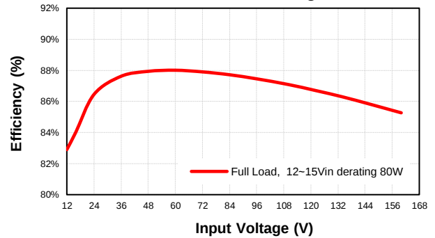
CQB100W14-72S12 Eff Vs Vin @25 Deg. C
