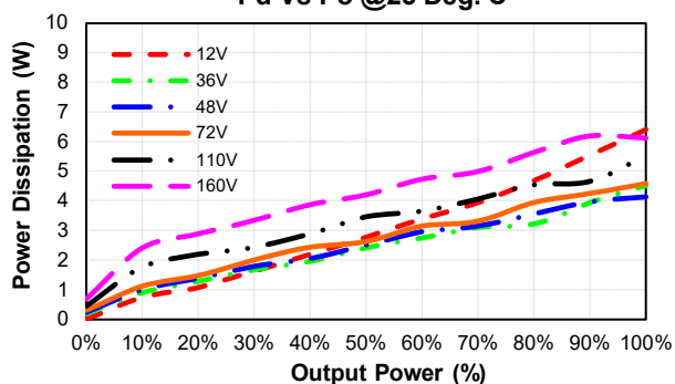
ECB40W18-72S54 Pd Vs Po @25 Deg. C
