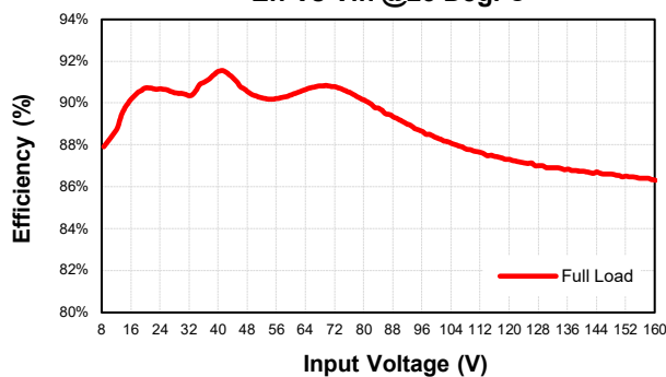
ECB40W18-72S12 Eff Vs Vin @25 Deg. C
