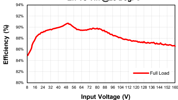
ECB40W18-72S24 Eff Vs Vin @25 Deg. C
