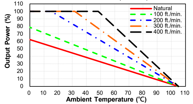
CQB150W14-72S12, 15, 28, 54 Derating Curve without Heatsink (Vin=72V)
