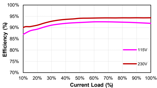
LFM420S240 (Eff Vs Io)
