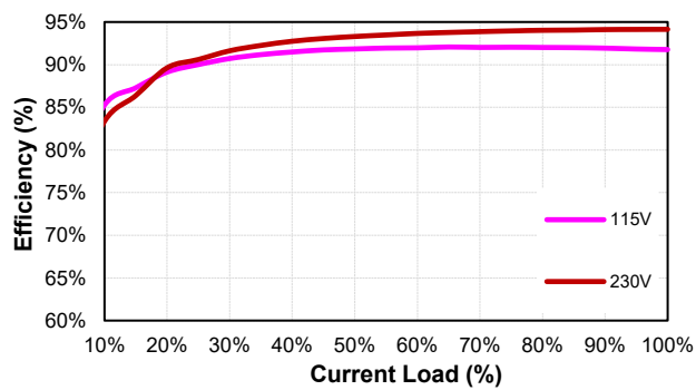
LFM300M540 (Eff Vs Io)
