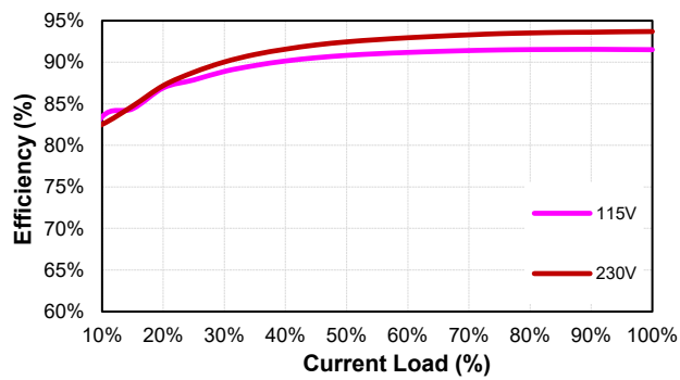
LFM300M300 (Eff Vs Io)
