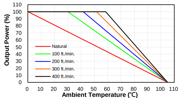
CQB150W8-36S24 Derating Curve with Heatsink QBL127 (Vin=36V)
