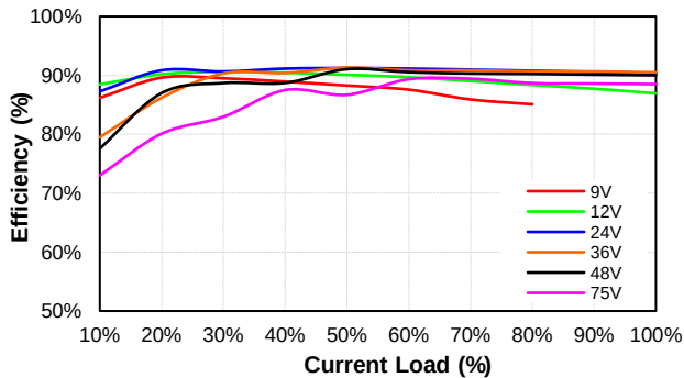
CQB150W8-36S54 Eff Vs Io @25 Deg. C
