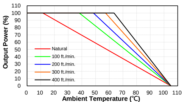
CQB150W8-36S12, 15, 28, 48, 54 Derating Curve with Heatsink QBL127 (Vin=36V)
