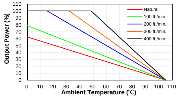
CQB150W18-36S12, 15, 28, 48, 54 Derating Curve without Heatsink (Vin=36V)
