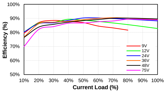
CQB150W8-36S05 Eff Vs Io @25 Deg. C
