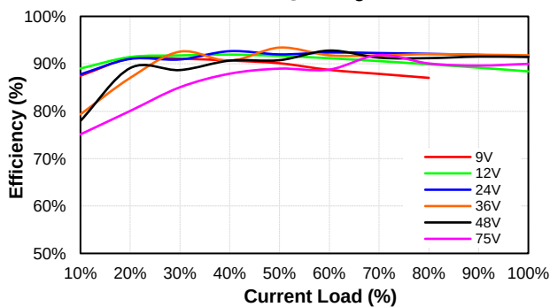
CQB150W8-36S15 Eff Vs Io @25 Deg. C
