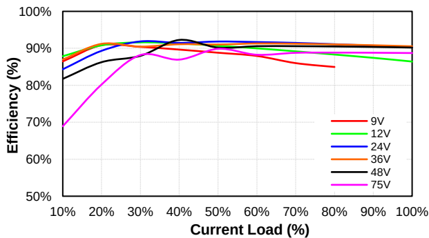
CQB150W8-36S12 Eff Vs Io @25 Deg. C
