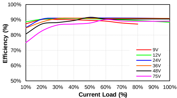
CQB150W8-36S28 Eff Vs Io @25 Deg. C
