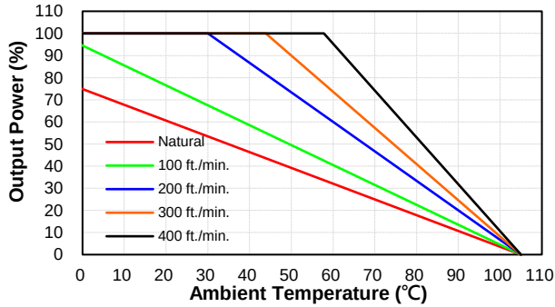
CQB150W8-36S05 Derating Curve without Heatsink (Vin=36V)
