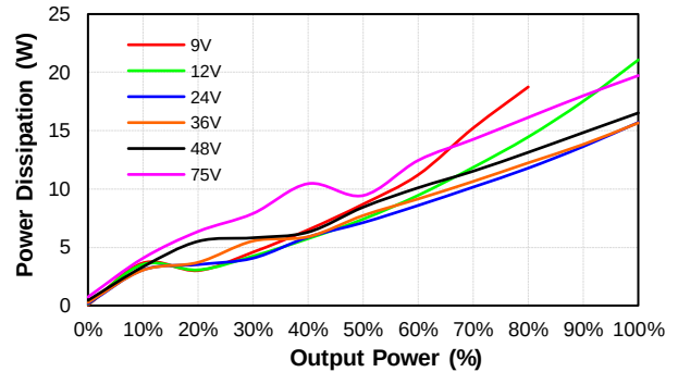
CQB150W8-36S48 Pd Vs Po @25 Deg. C
