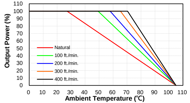
CQB150W8-36S05 Derating Curve with Heatsink QBL127 (Vin=36V)
