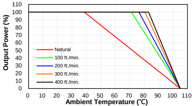
CQB150W8-36S05 Derating Curve with Heatsink QBT210 (Vin=36V)
