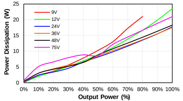
CQB150W8-36S24 Pd Vs Po @25 Deg. C
