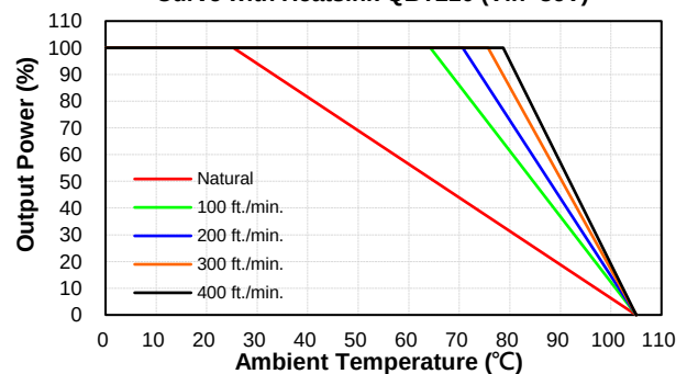
CQB150W8-36S12, 15, 28, 48, 54 Derating Curve with Heatsink QBT210 (Vin=36V)
