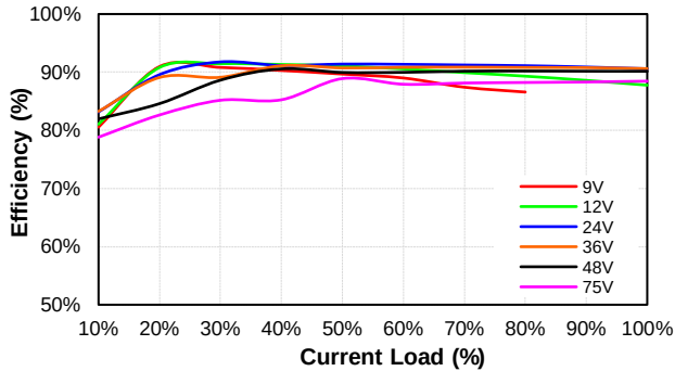
CQB150W8-36S48 Eff Vs Io @25 Deg. C
