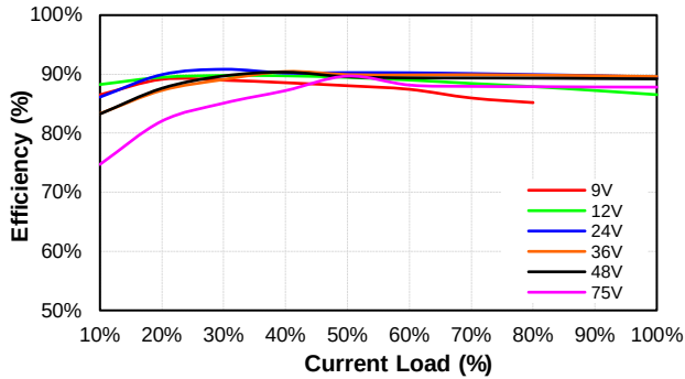
CQB150W8-36S24 Eff Vs Io @25 Deg. C
