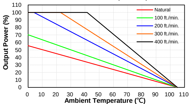
CQB150W8-36S24 Derating Curve without Heatsink (Vin=36V)
