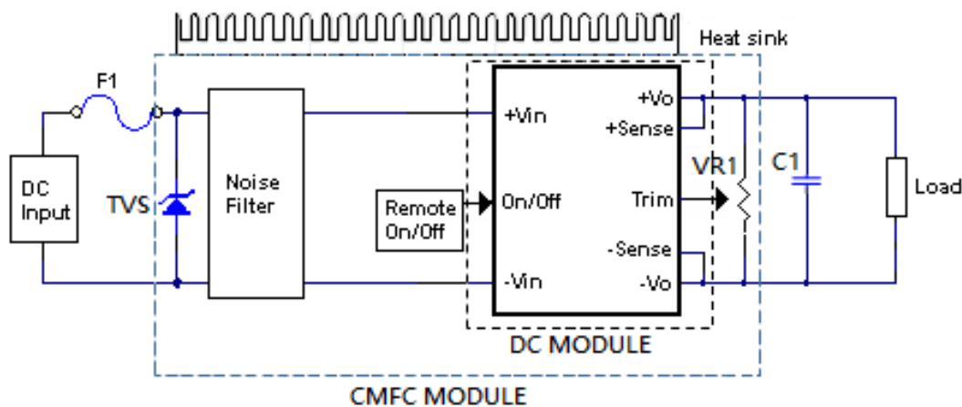
Connection circuit for conducted EMI testing
