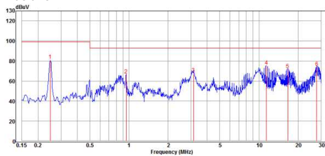
CQB50W12-72S24-CMFC
