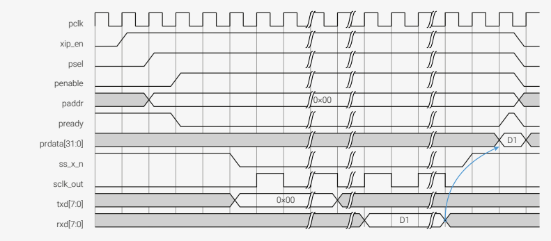
Figure 159. Typical Read Operation in XIP Mode
