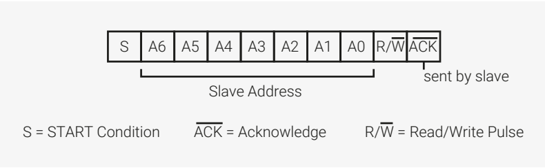
Figure 65. I2C 7-bit Address Format
