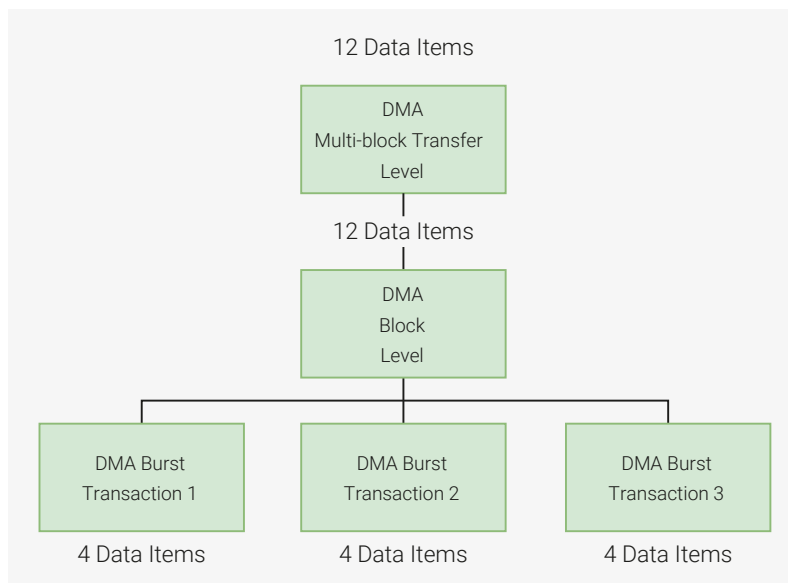
Figure 160. Breakdown of DMA Transfer into Burst Transactions. Block size, DMA.CTLx.BLOCKS\_TS = 12 . Number of data items per source burst transaction, DMA.CTLx.SRC\_MSIZE = 4 . SSI receive FIFO watermark level, SSI.DMARDLR + 1 = DMA.CTLx.SRC\_MSIZE = 4
