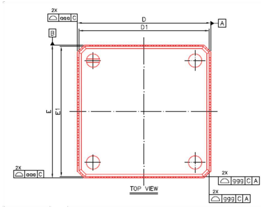
Figure 3-12 Top View
