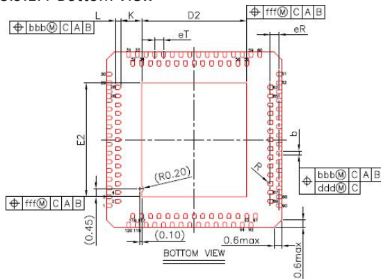
Figure 3-11 Bottom view
