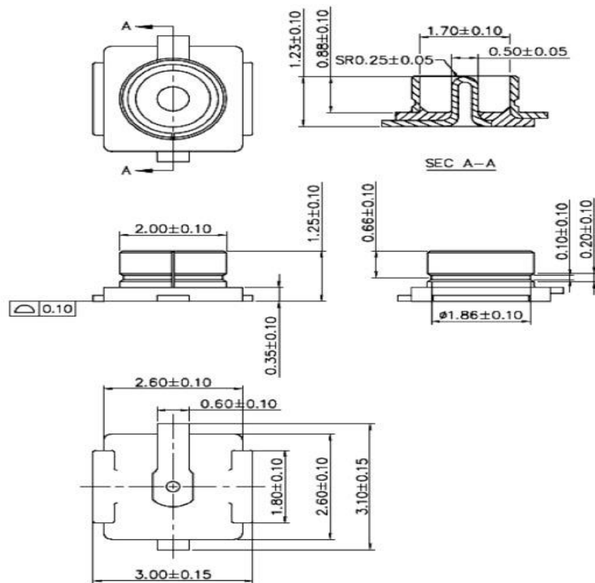
Figure 7 Size of External Antenna Connector
