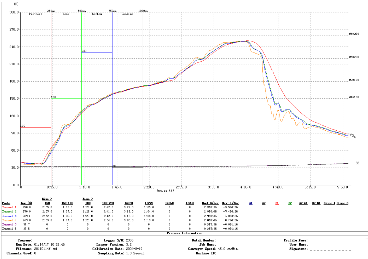
Figure 11 Temperature Curve of Secondary Reflow
