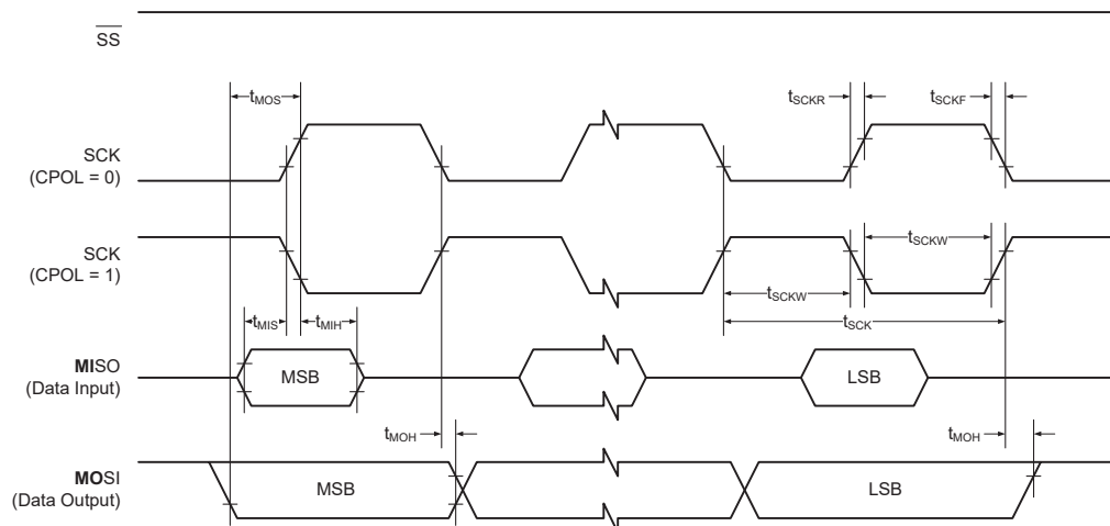
Figure 38-5. SPI - Timing Requirements in Master Mode
