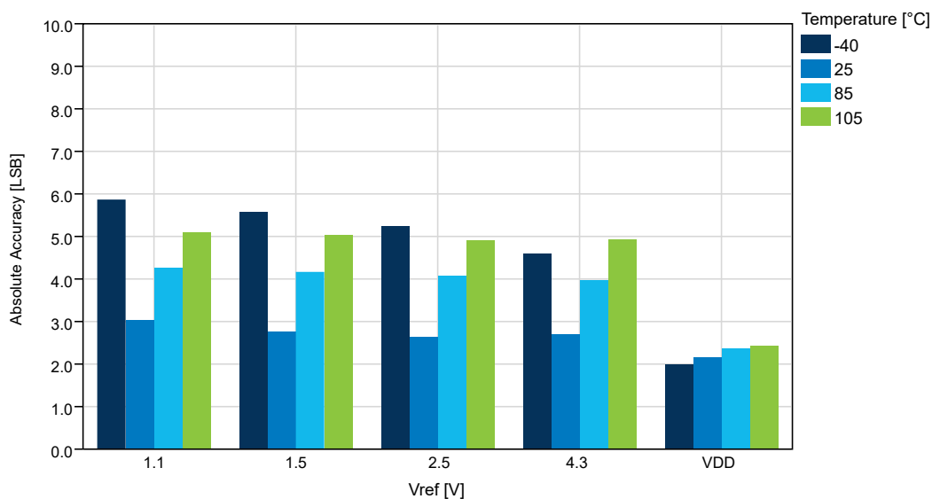
Figure 39-38. Absolute Accuracy vs. V_{ref} ( V_{DD}=5.0\text{V} , f_{ADC}=115 ksp/s), REFSEL = Internal Reference
