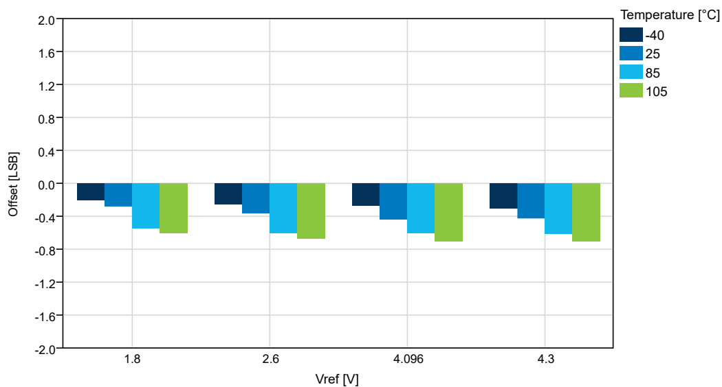
Figure 39-56. Offset vs. V_{REF} ( V_{DD}=5.0\text{V} , f_{ADC}=115 kps, REFSEL = External Reference)
