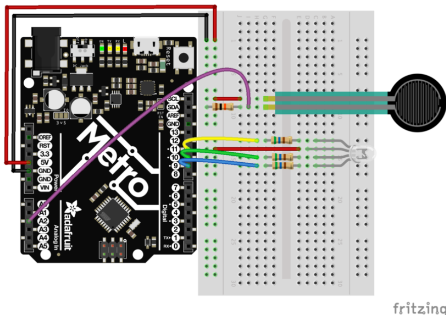
Diagram: RGB + Force Resistor
