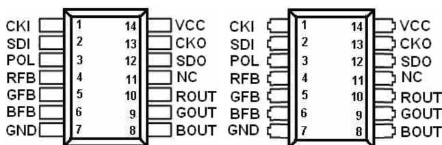
Fig1.a SOP-14 package
