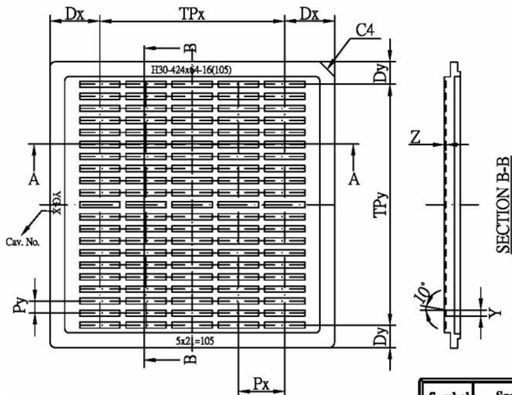
Figure 15-2: SSD1351UR1 Die Tray Information
