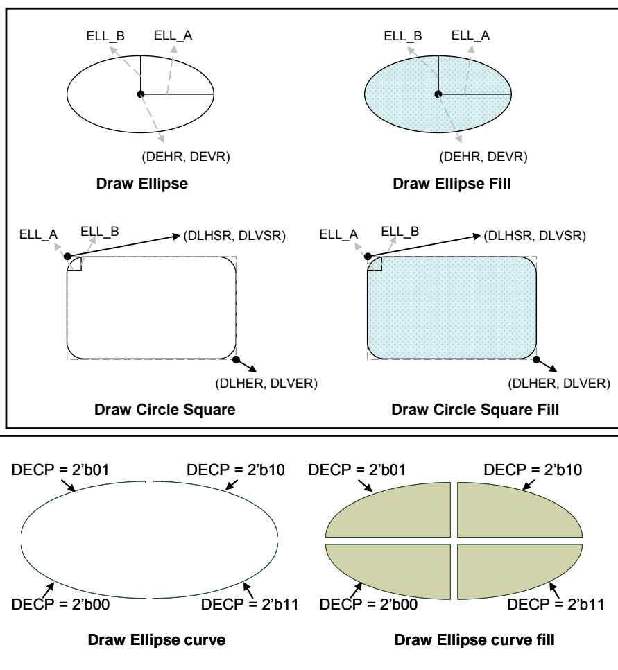
Figure 5-7 : The Drawing Function
