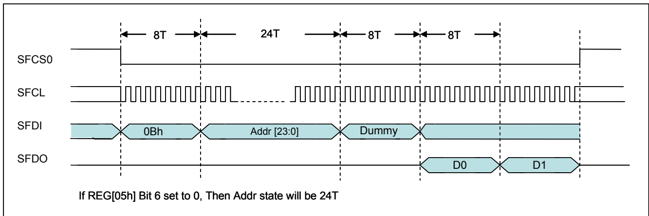
Figure 6-38 : 5-BUS (Fast) Read
