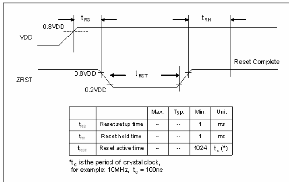
Figure 6-50 : Reset Timing
