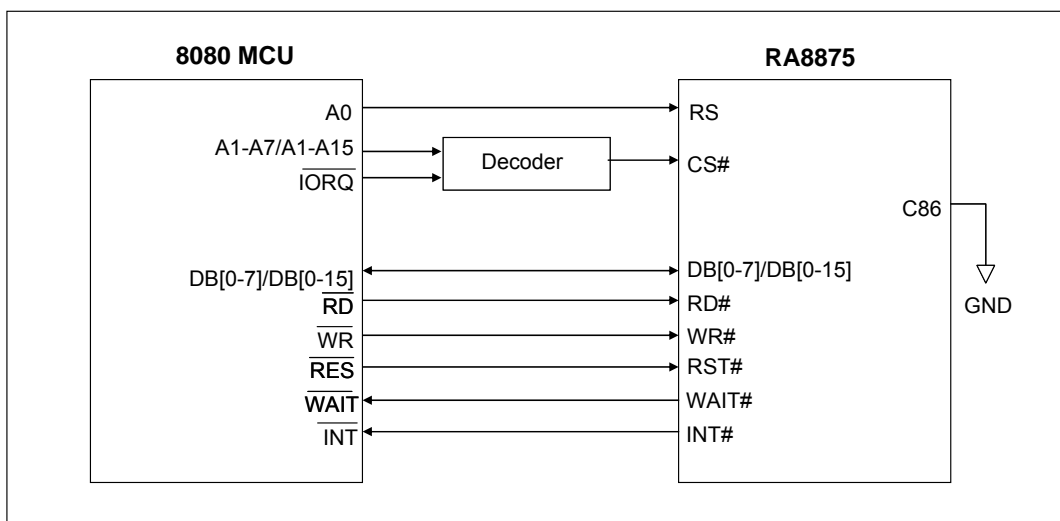
Figure 6-1 : 8080 MCU Interface
