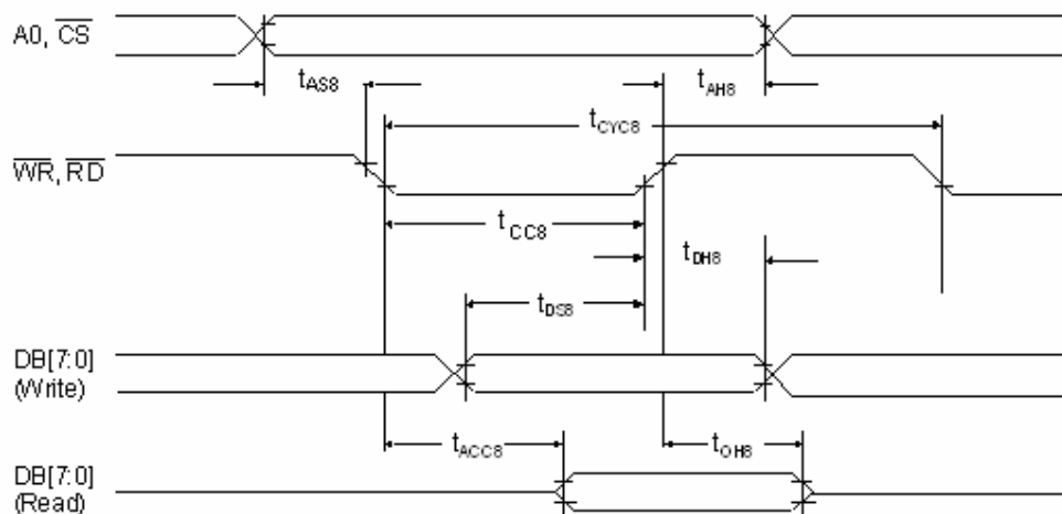
Figure 6-4 : 8080 Waveform
