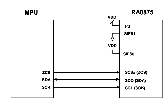
Figure 6-7 : The MCU Interface Diagram of 3-Wire SPI
