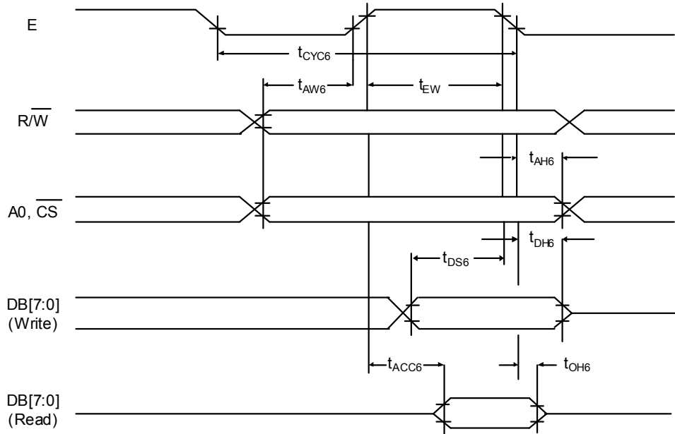
Figure 6-3 : 6800 MCU Waveform
