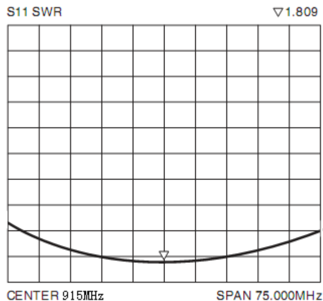
Typical VSWR
