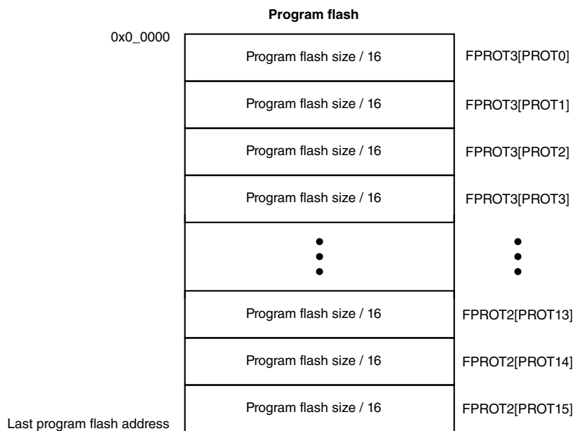
Figure 32-4. Program flash protection (512KB or 1MB of program flash)
