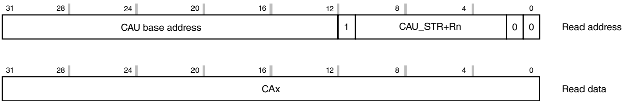
Figure 37-6. Indirect store
