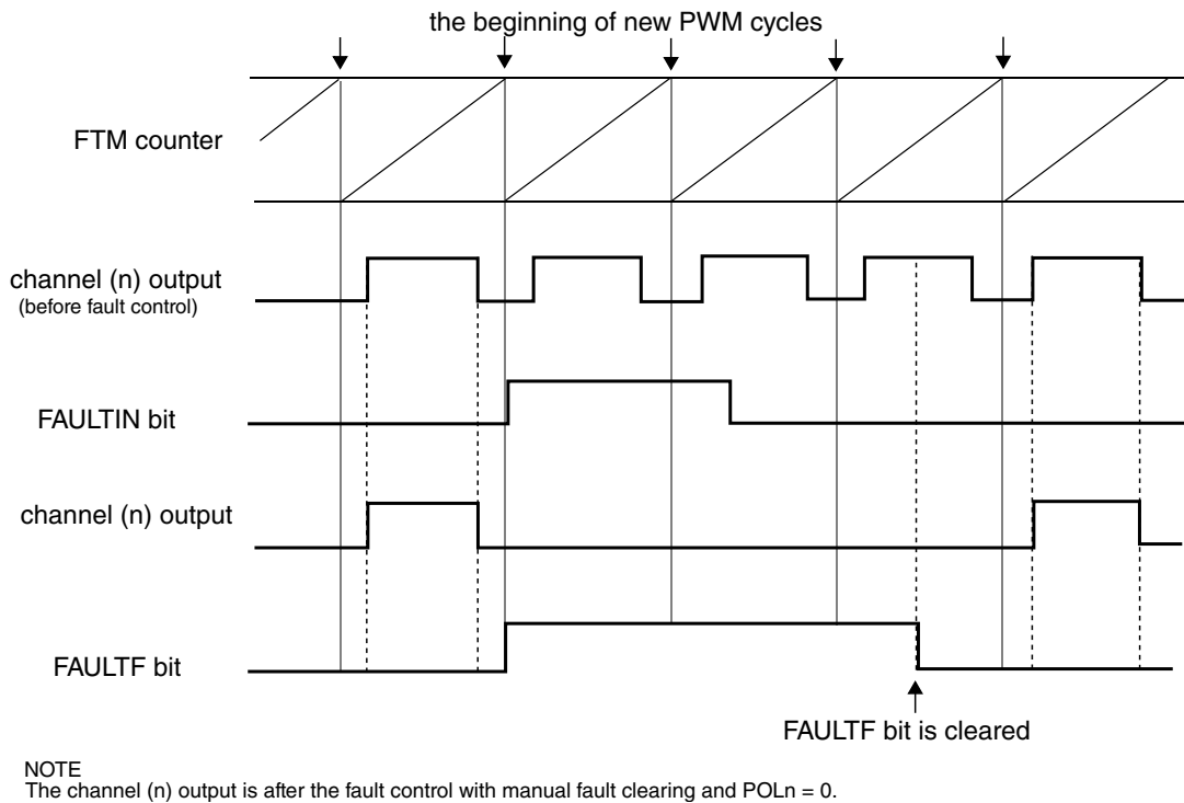
Figure 45-74. Fault control with manual fault clearing
