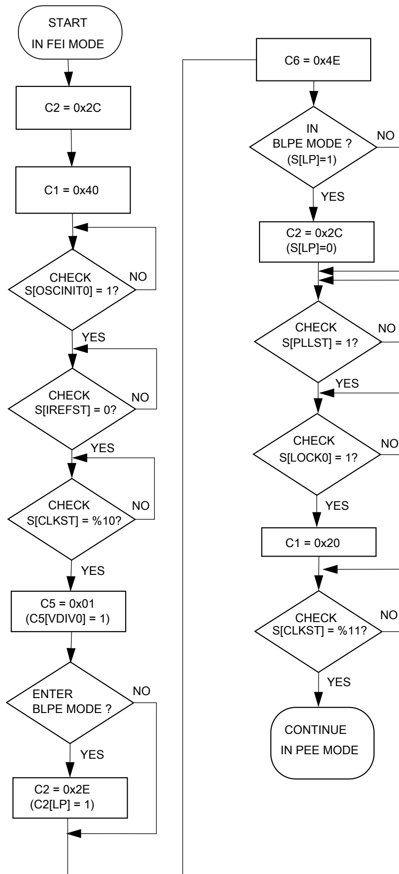
Figure 27-3. Flowchart of FEI to PEE mode transition using a 16 MHz crystal K66 Sub-Family Reference Manual, Rev. 4, August 2018
