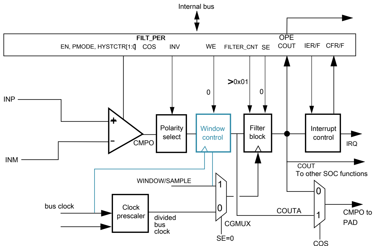
Figure 40-7. Scaled, Filtered (# 4B): sampling point internally derived
