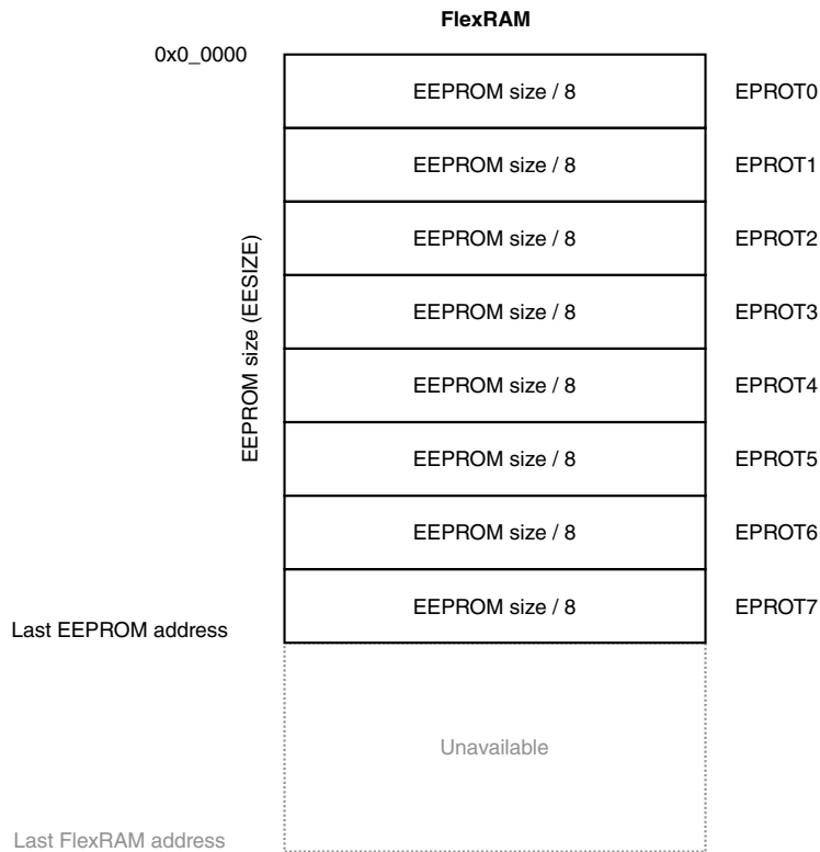
Figure 32-8. EEPROM protection
