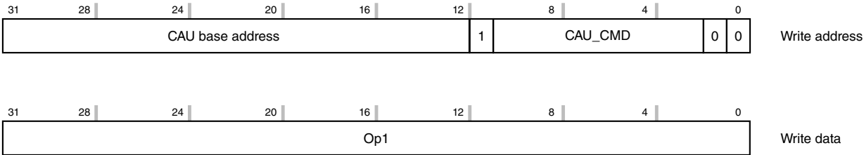
Figure 37-5. Indirect loads
