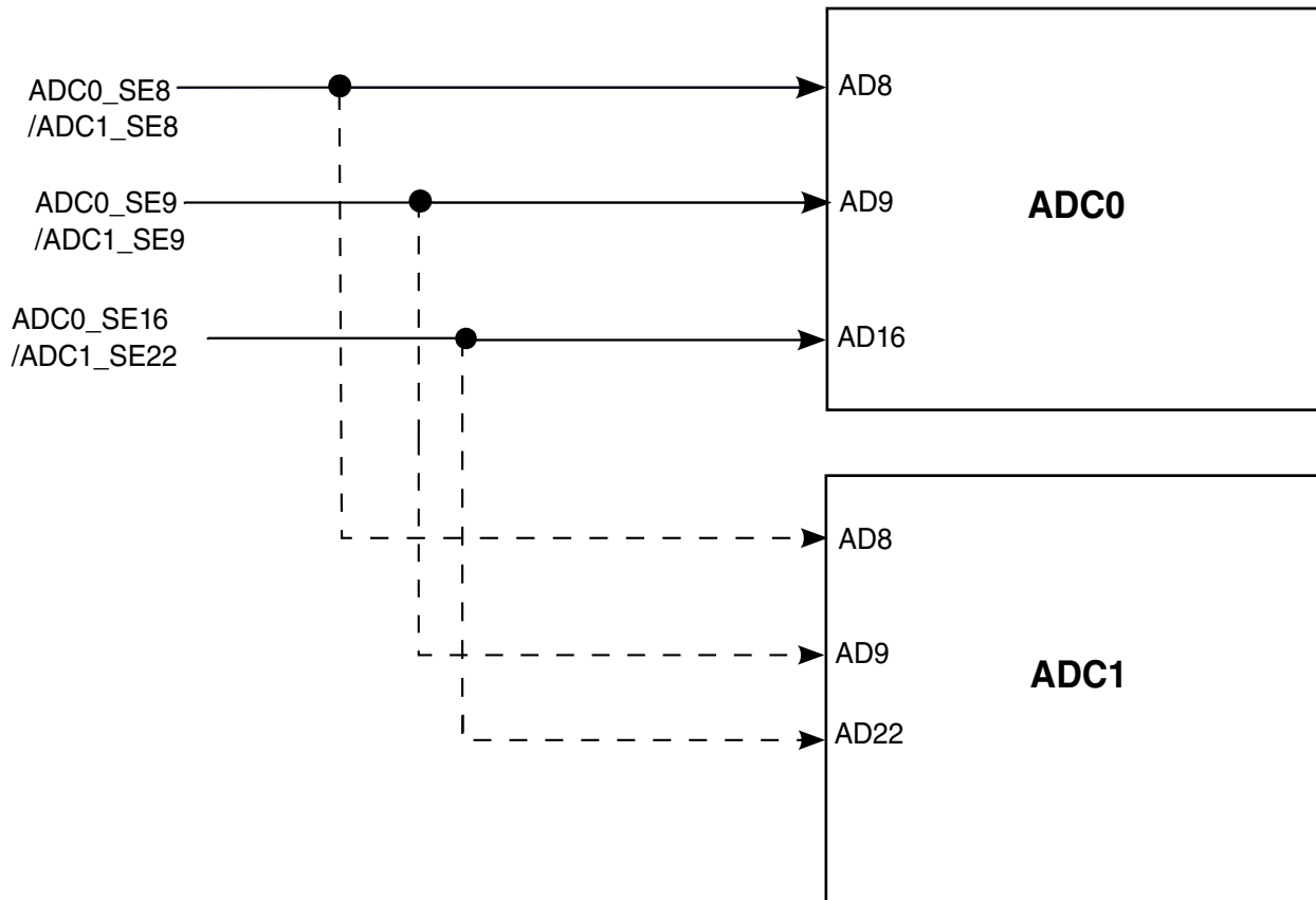
Figure 39-2. ADC hardware interleaved channels integration
