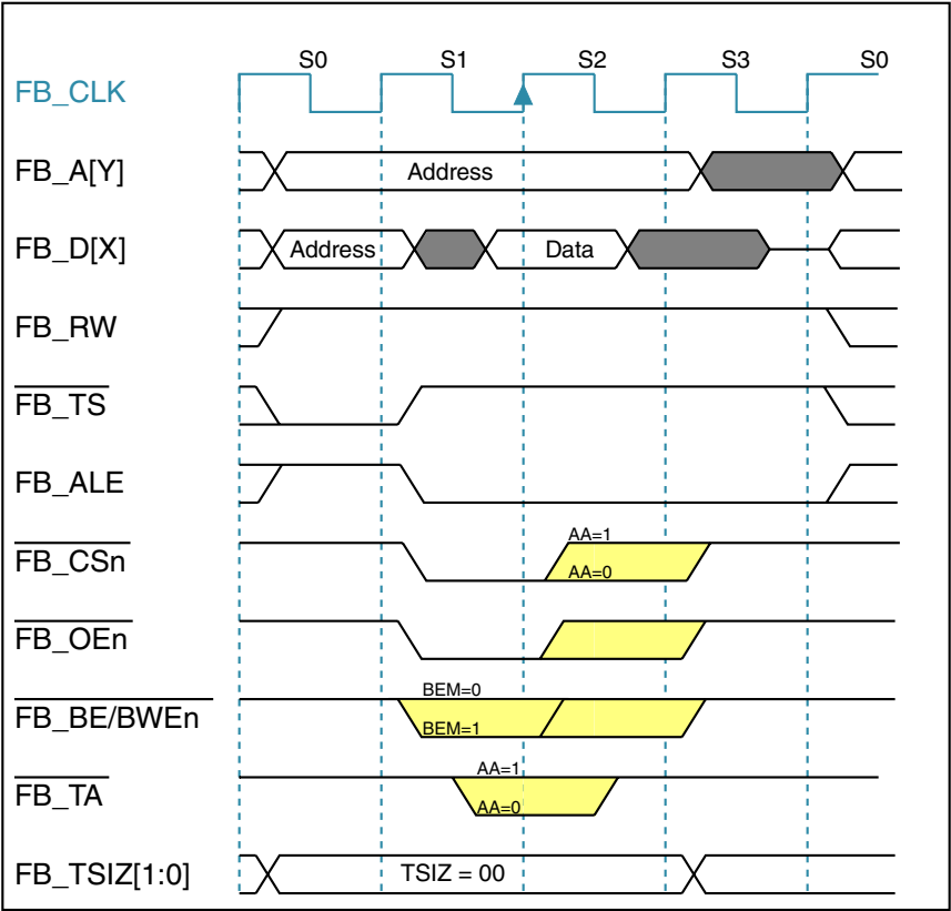
Figure 34-12. Longword-Read Transfer
