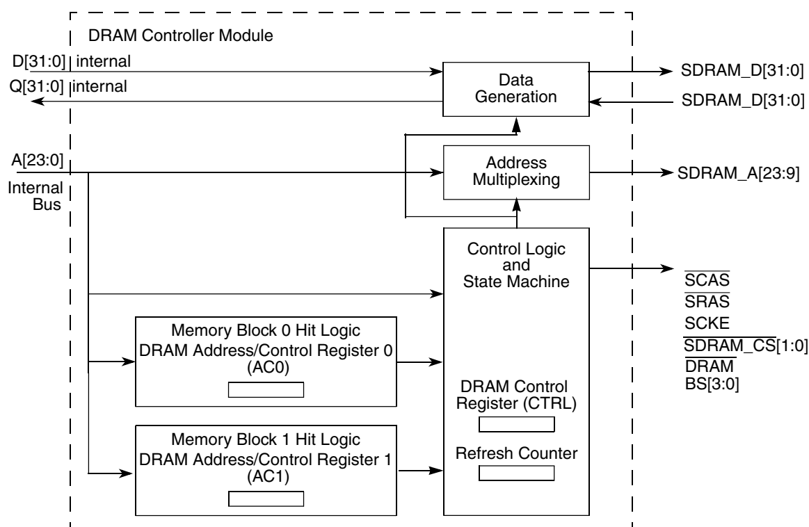
Figure 35-1. Block diagram
