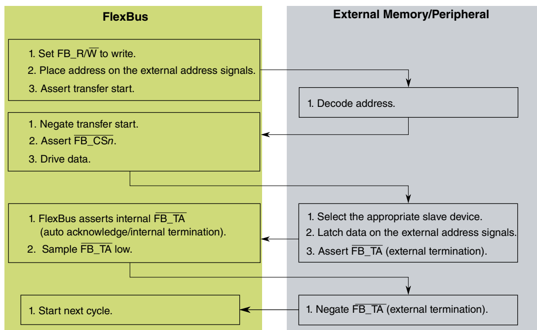
Figure 34-6. Write-Cycle Flowchart
