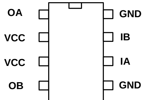
Device pins Figure
