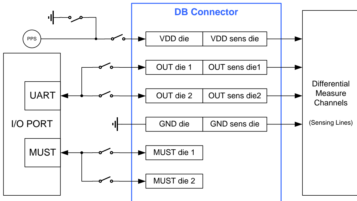
Figure 1: Functional Diagram
