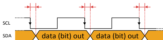
Figure 24: TrimDelSDAOut Definition
