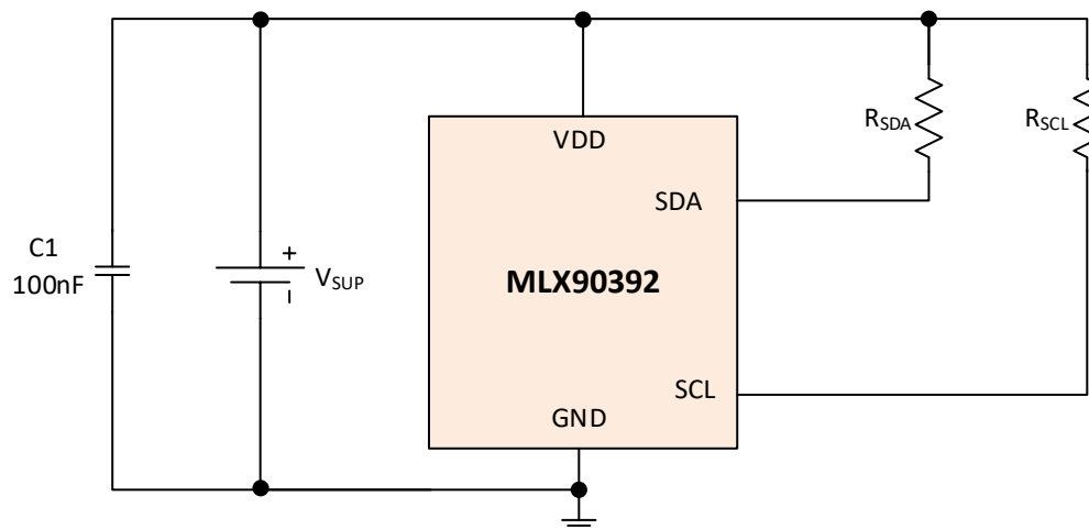
Figure 22: Recommended application diagram
