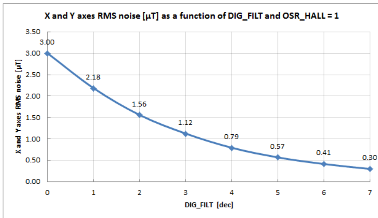
Figure 14: version 010 - XY axis RMS noise (typ)
