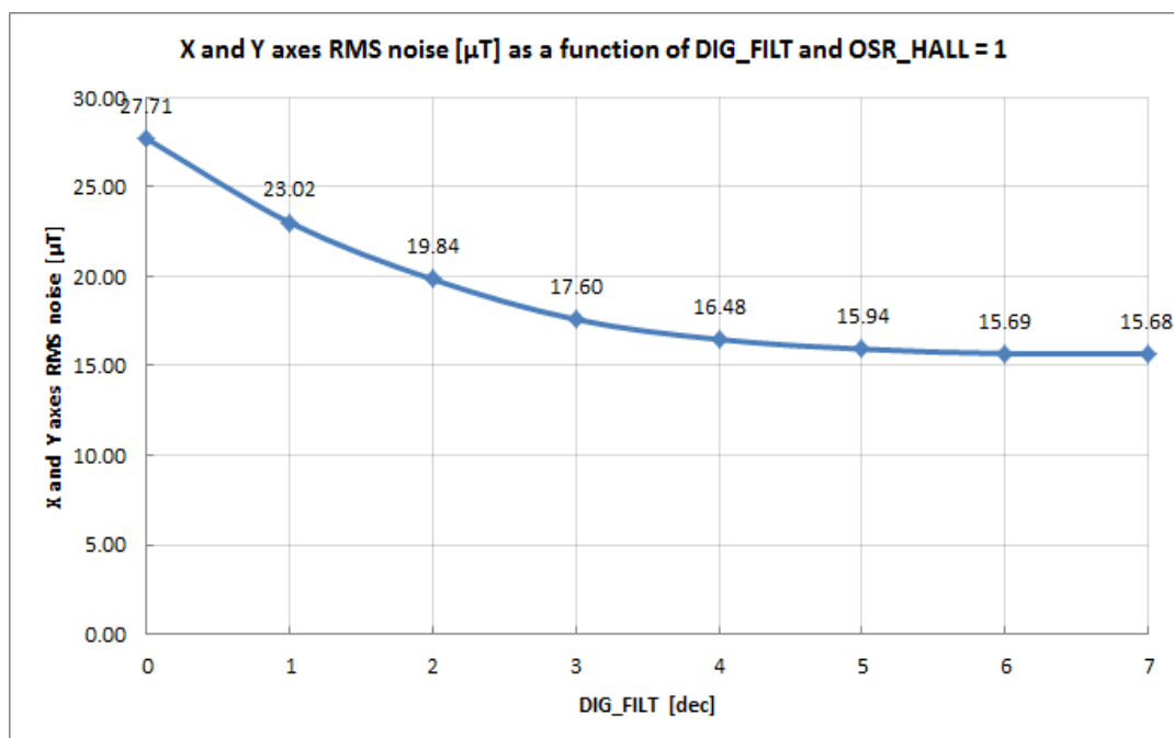
Figure 20: version 011 - XY axis RMS noise (typ)
