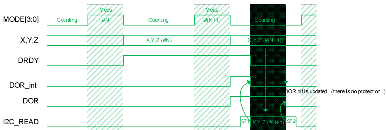
Figure 9: Data Skip: When data is not read
