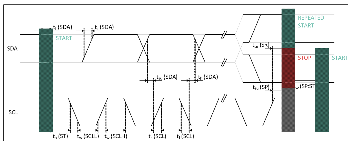
Figure 2: I 2 C Timing Diagram
