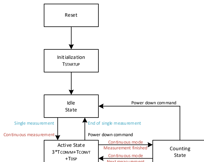
Figure 13: Sequence flowchart
