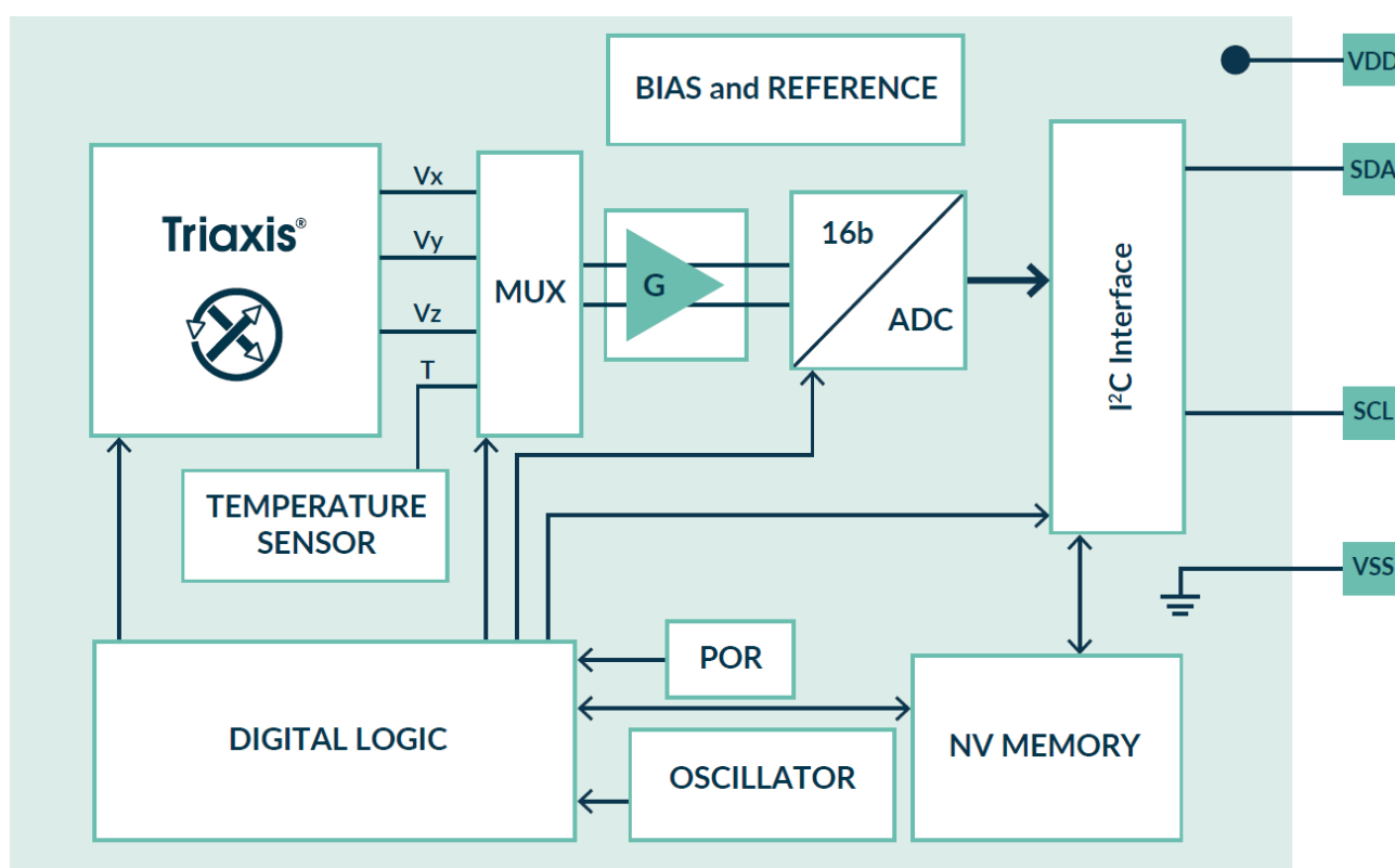
Figure 1: IC block diagram
