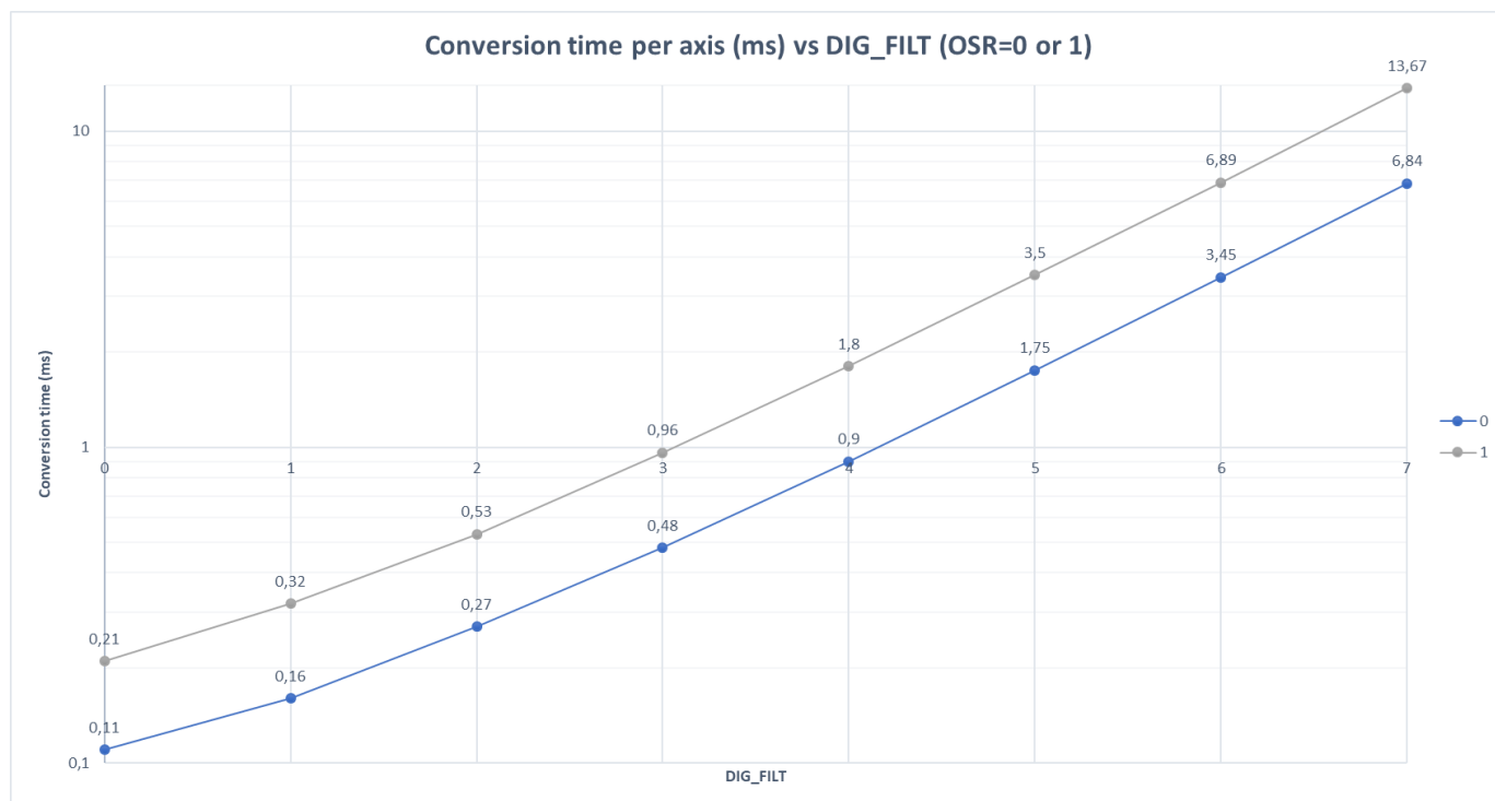
Figure 3: Conversion time
