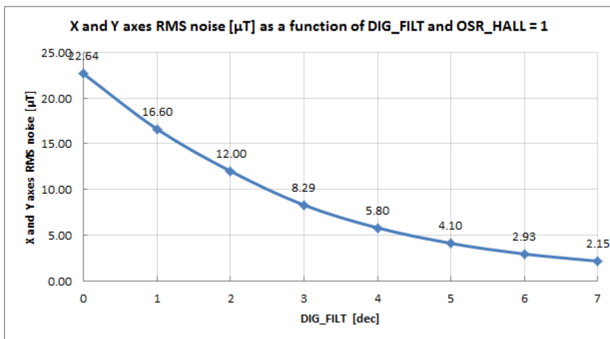
Figure 18: version 011 – XY axis RMS noise (typ)
