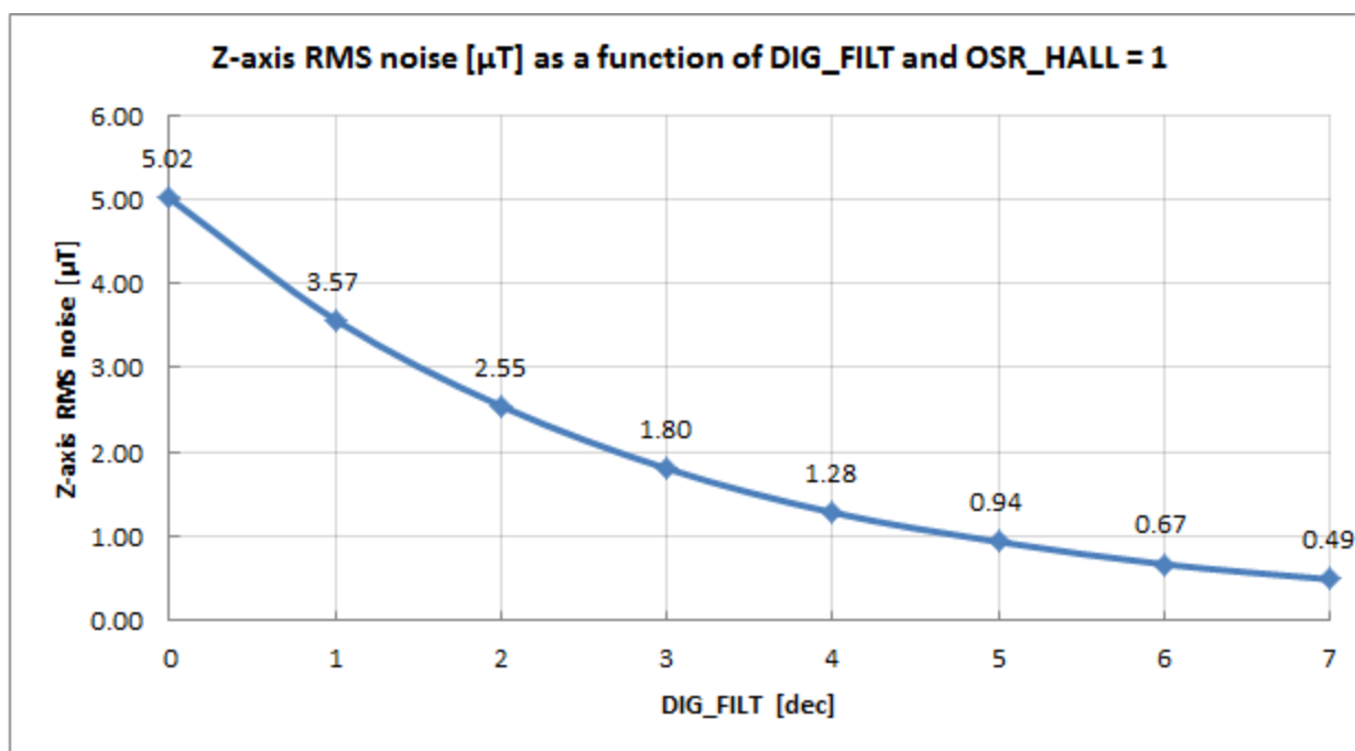
Figure 15: version 010 - Z axis RMS Noise (typ)
