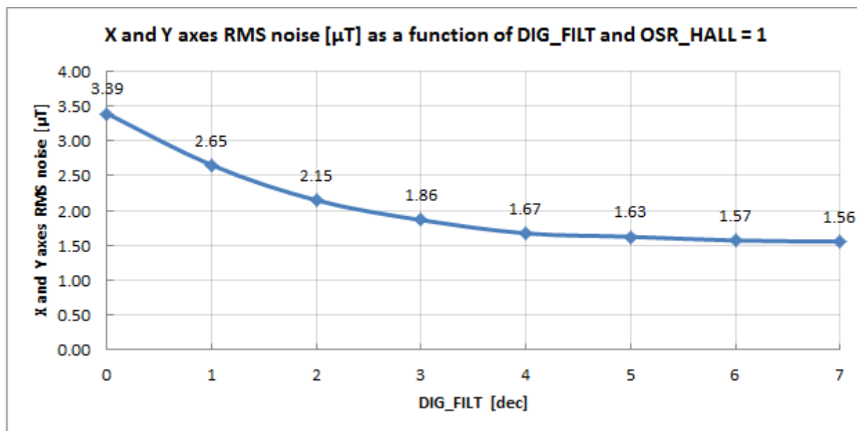
Figure 16: version 010 - XY axes RMS noise(typ)
