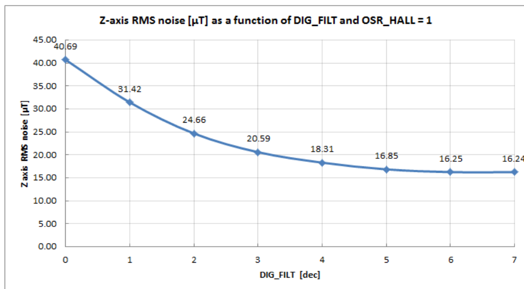
Figure 21: version 011 - Z axis RMS noise (typ)
