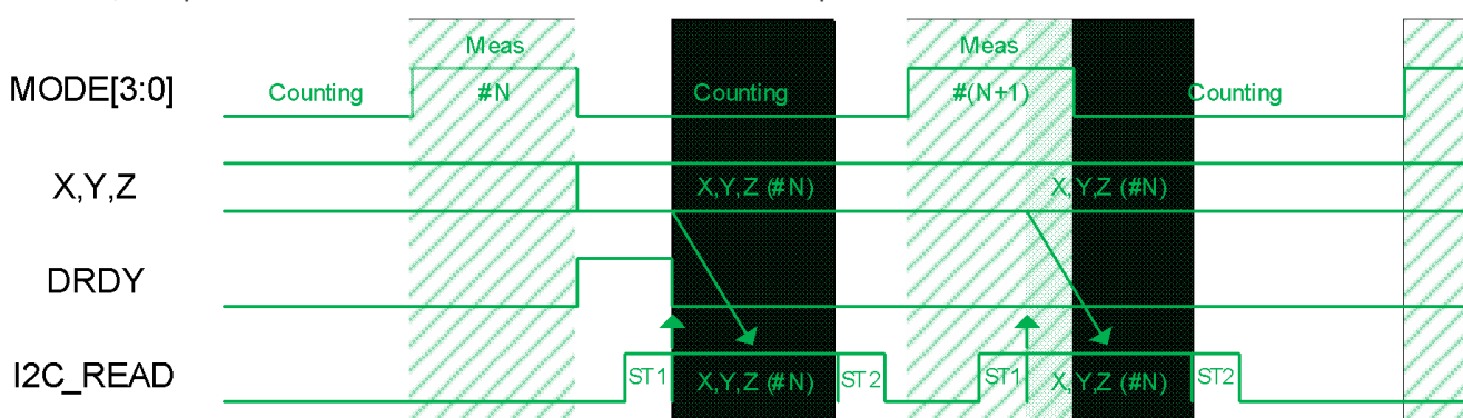
Figure 8: Data read start during measurement
