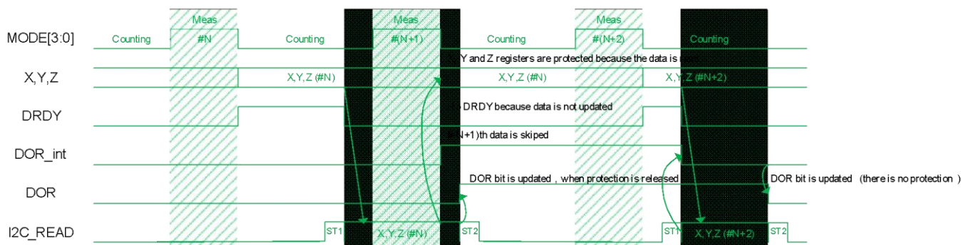
Figure 10: Data Skip: When data read has not been finished before the next measurement end
