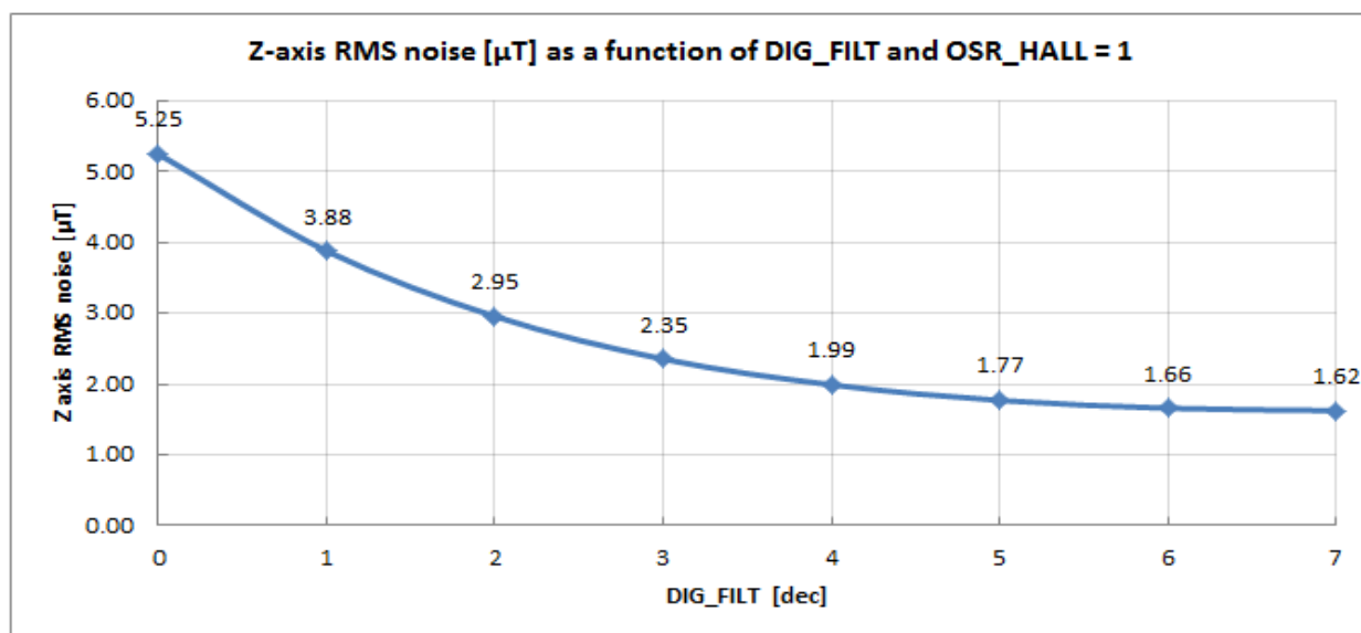
Figure 17: version 010 - Z axis RMS noise (typ)
