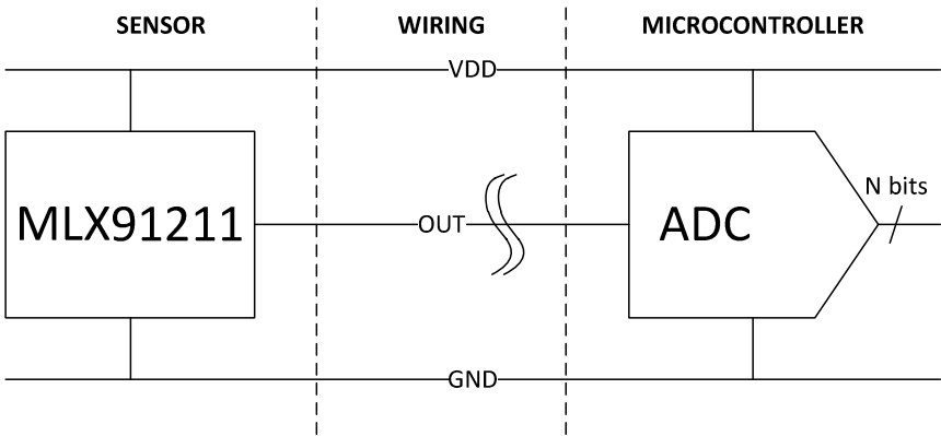
Figure 2 Ratiometry Application
