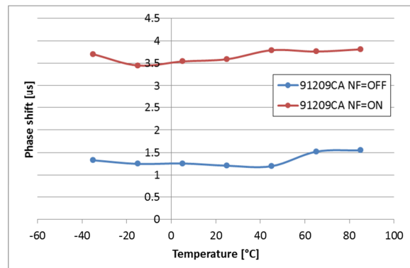
Figure 9: Phase shift over temperature.
