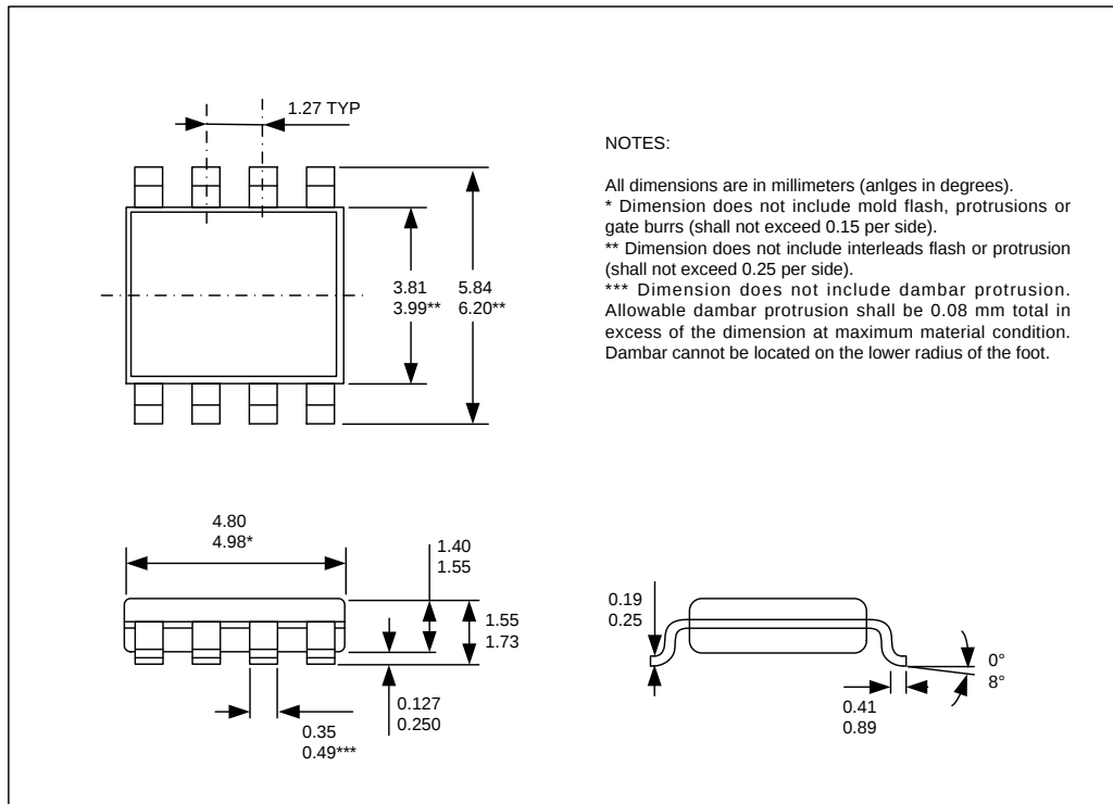
Figure 8: Package dimensions
