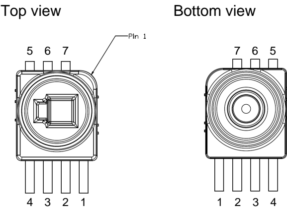
Figure 3: Package pinout
