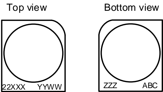
Figure 4: Package marking
