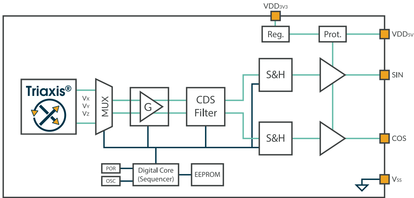
Figure 3: Functional Diagram
