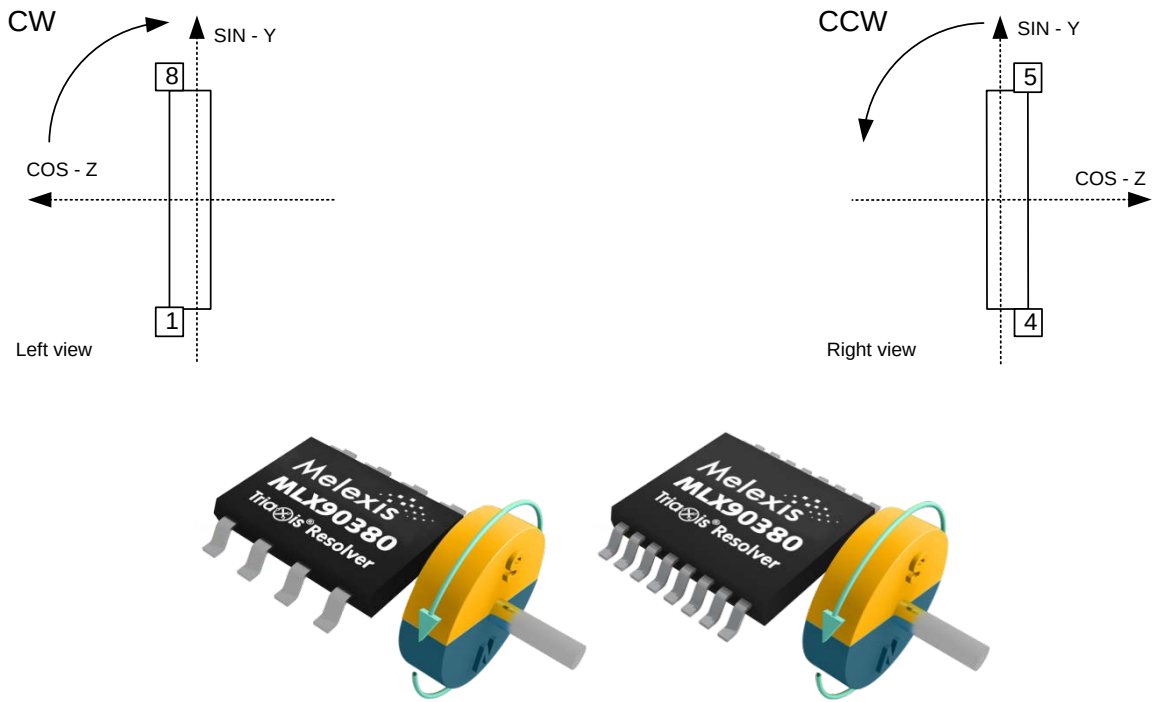
Figure 8: Z/Y Magnetic Axis
