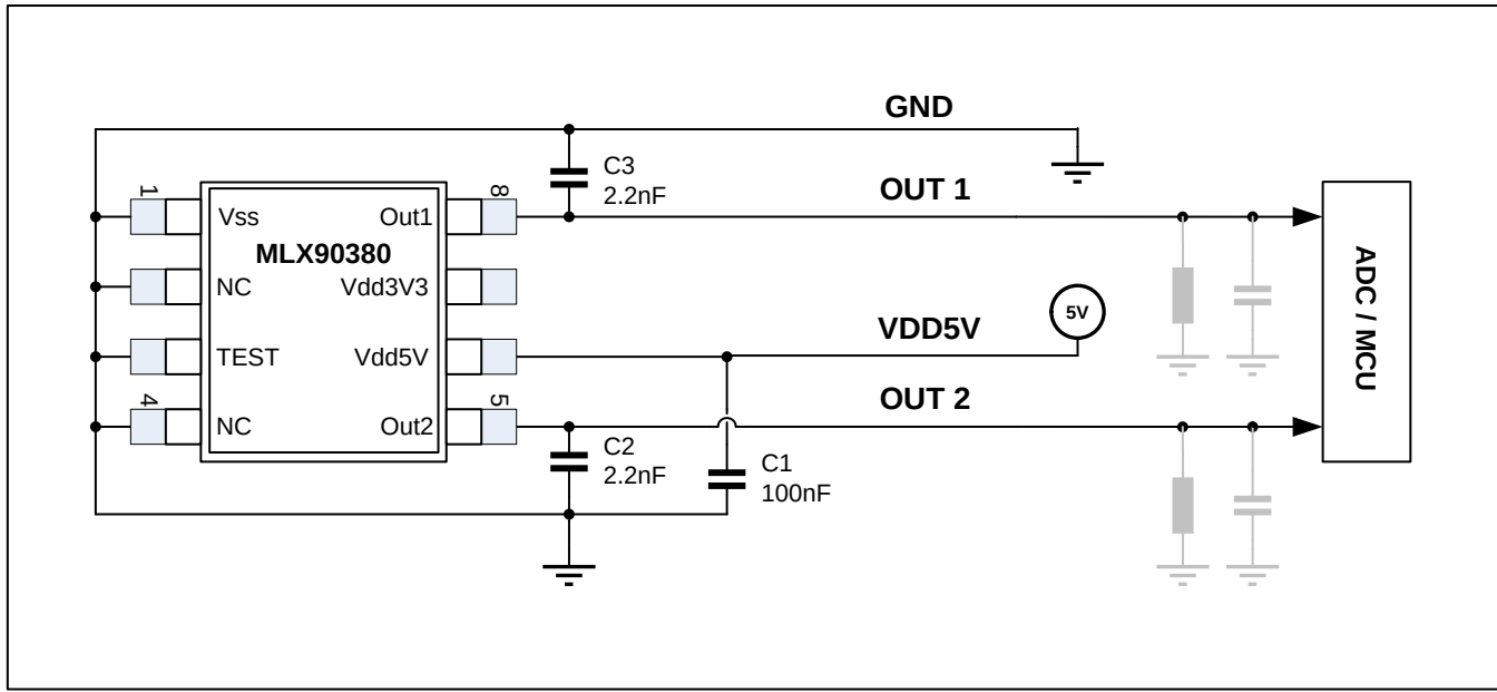
Figure 13: Application Diagram VDD5V
