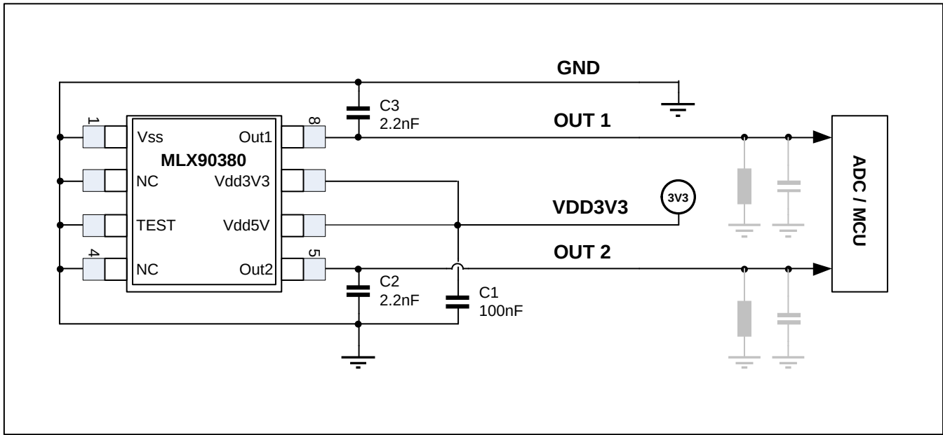
Figure 12: Application Diagram VDD3V3
