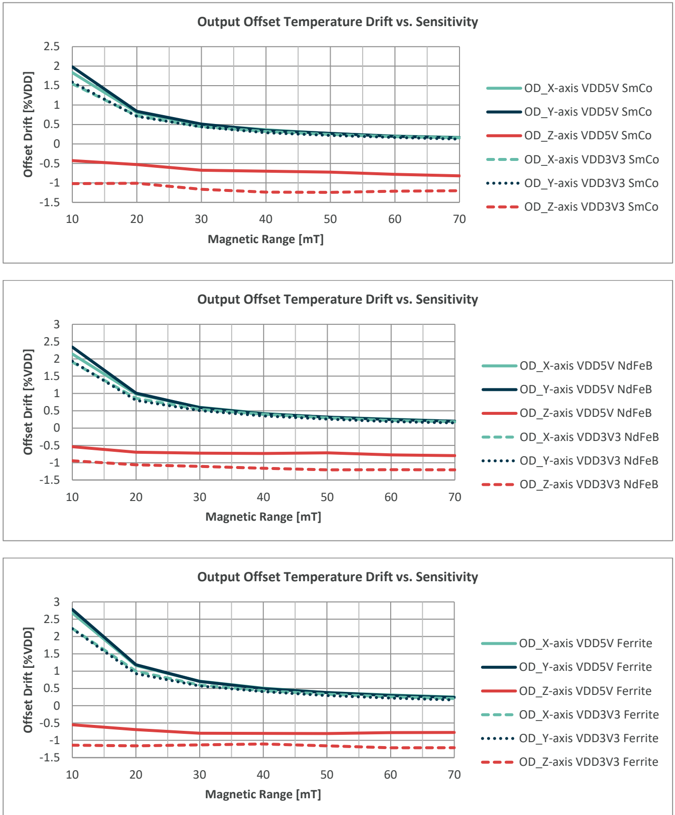
Figure 11: Output Offset Temperature Drift vs Sensitive Range per Magnet Type
