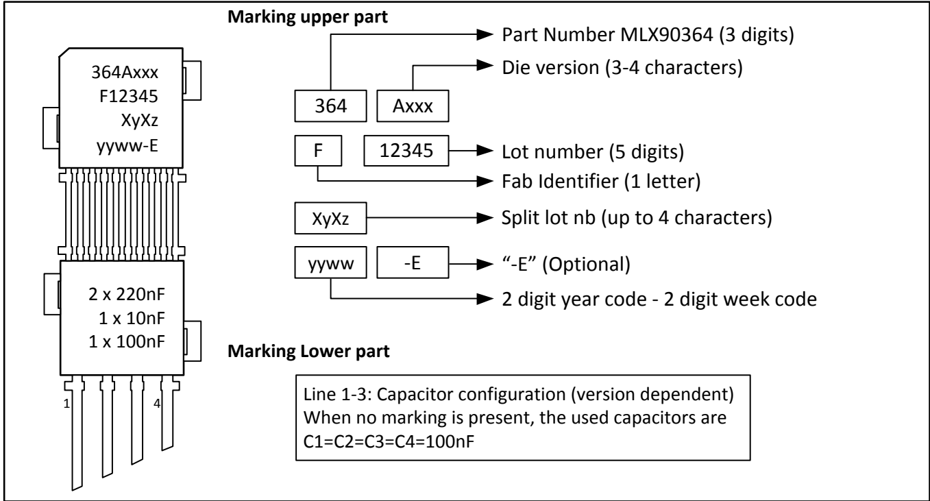
Figure 14 – DMP-4 marking convention
