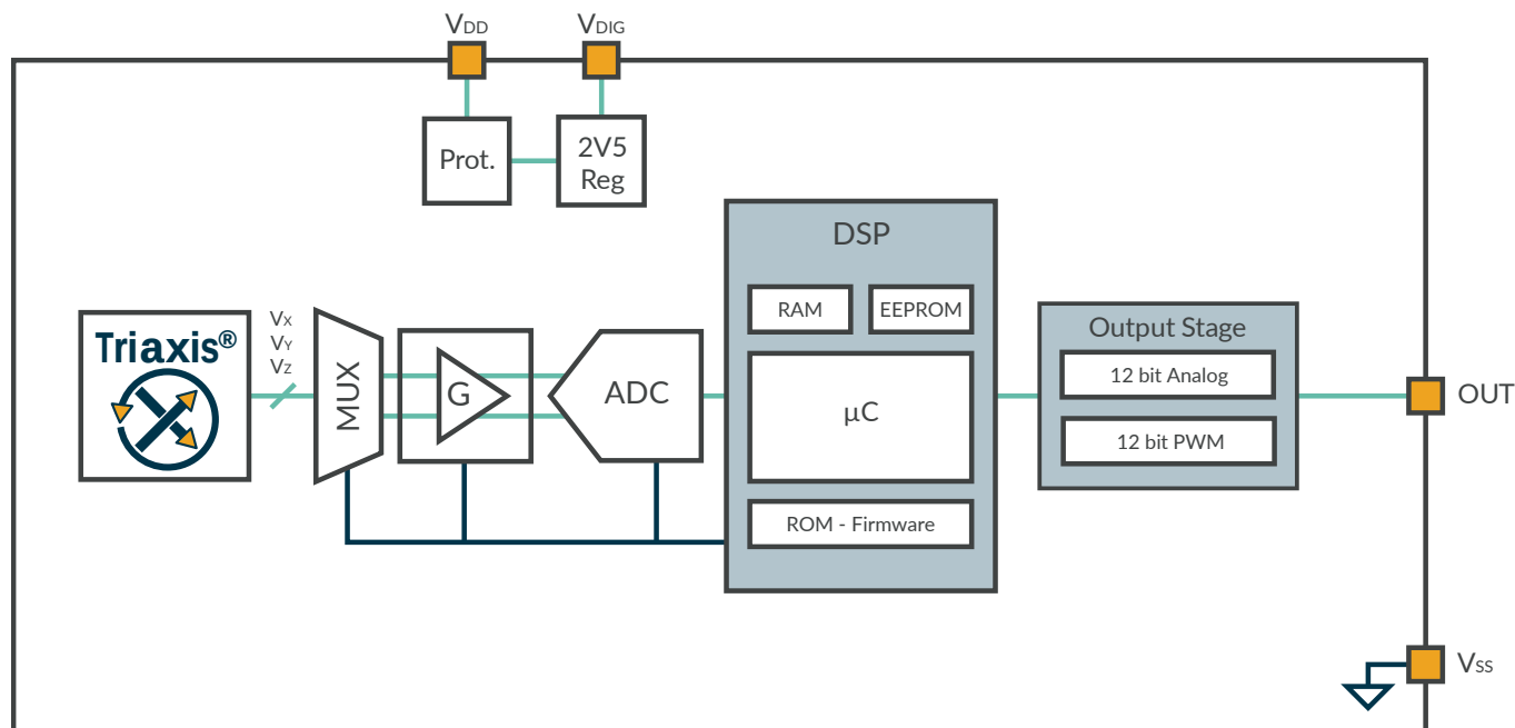
Figure 1 – Block Diagram
