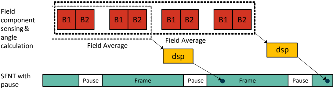
Figure 7 - Latency - Case FILTER = 2
