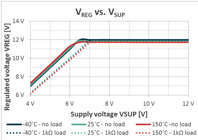
Figure 10-10 MLX83202 Regulated output voltage vs. supply voltage
