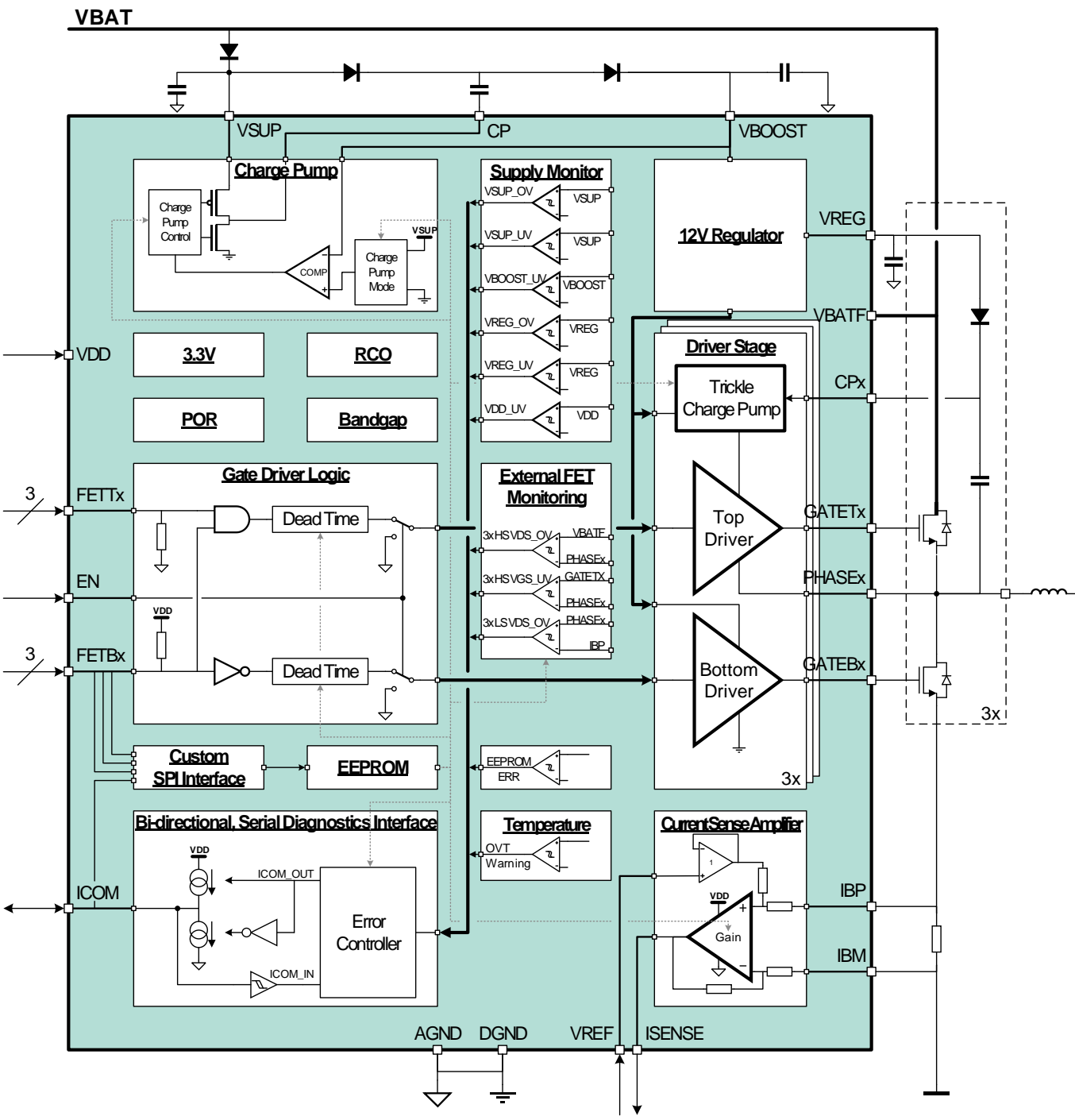
Figure 11-1 Block diagram
