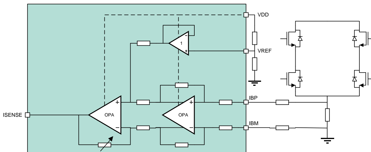
Figure 12-6 Current Sense Amplifier
