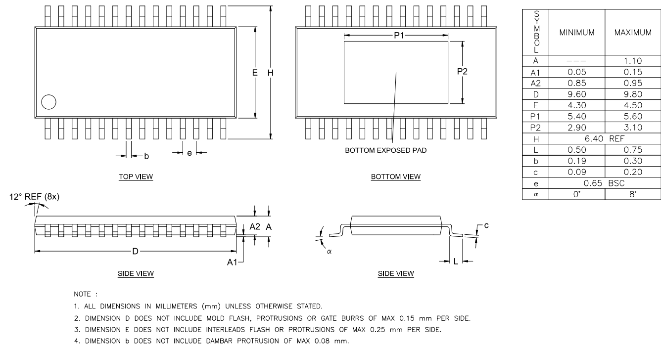
Figure 14-2 Package drawing & dimensions
