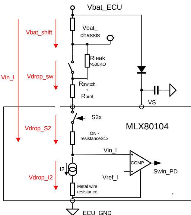
Figure 9 - Voltage drops external HS switch
