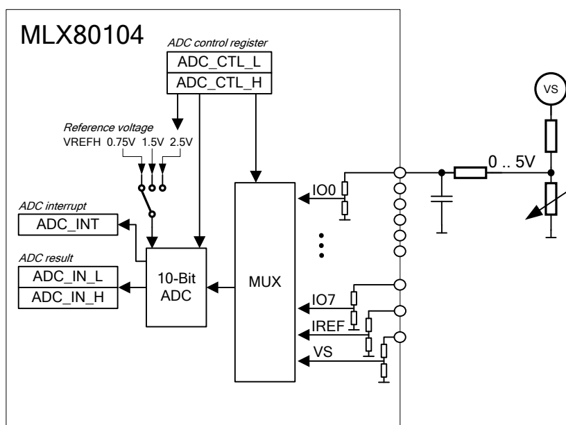
Figure 15 - ADC components
