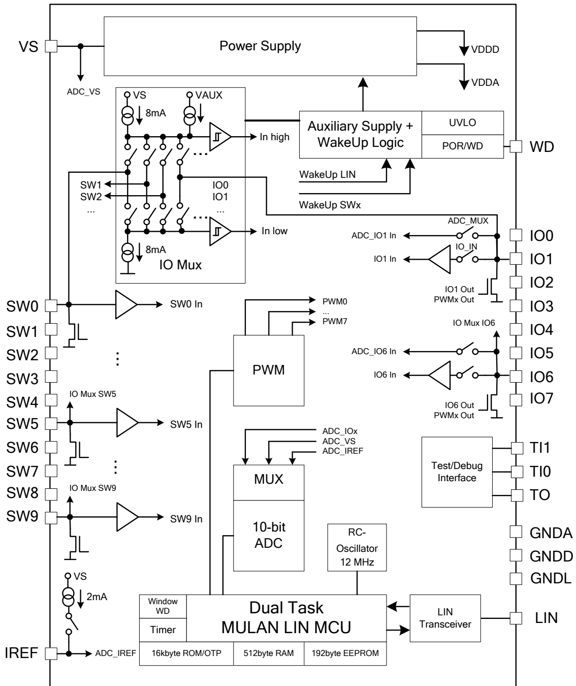
Figure 1 - Block Diagram
