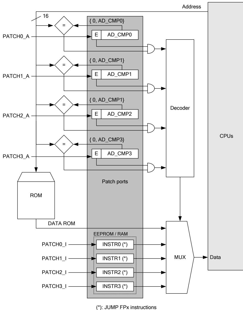
Figure 21 - Patch hardware
