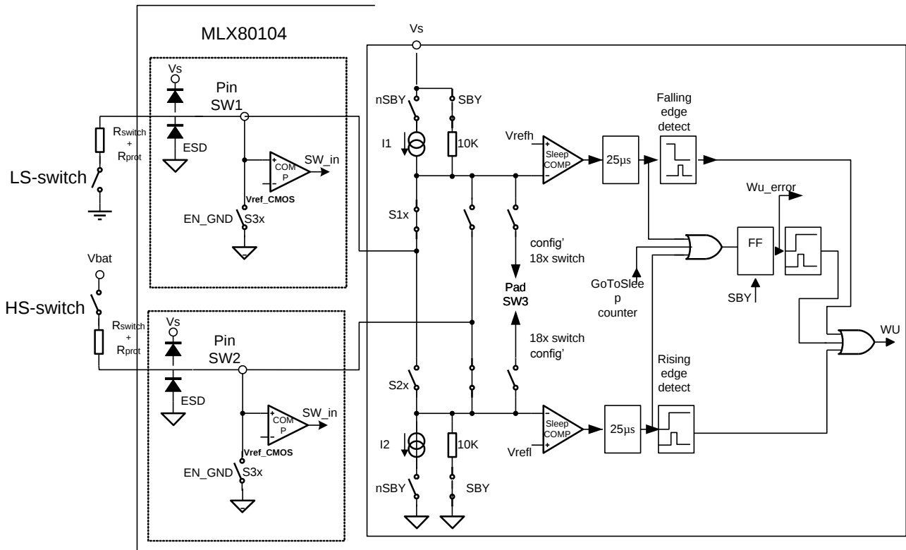
Figure 10 - Wake up detection for switch inputs
