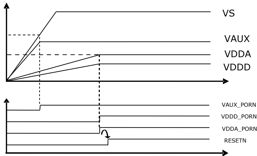
Figure 20 - Reset behaviour
