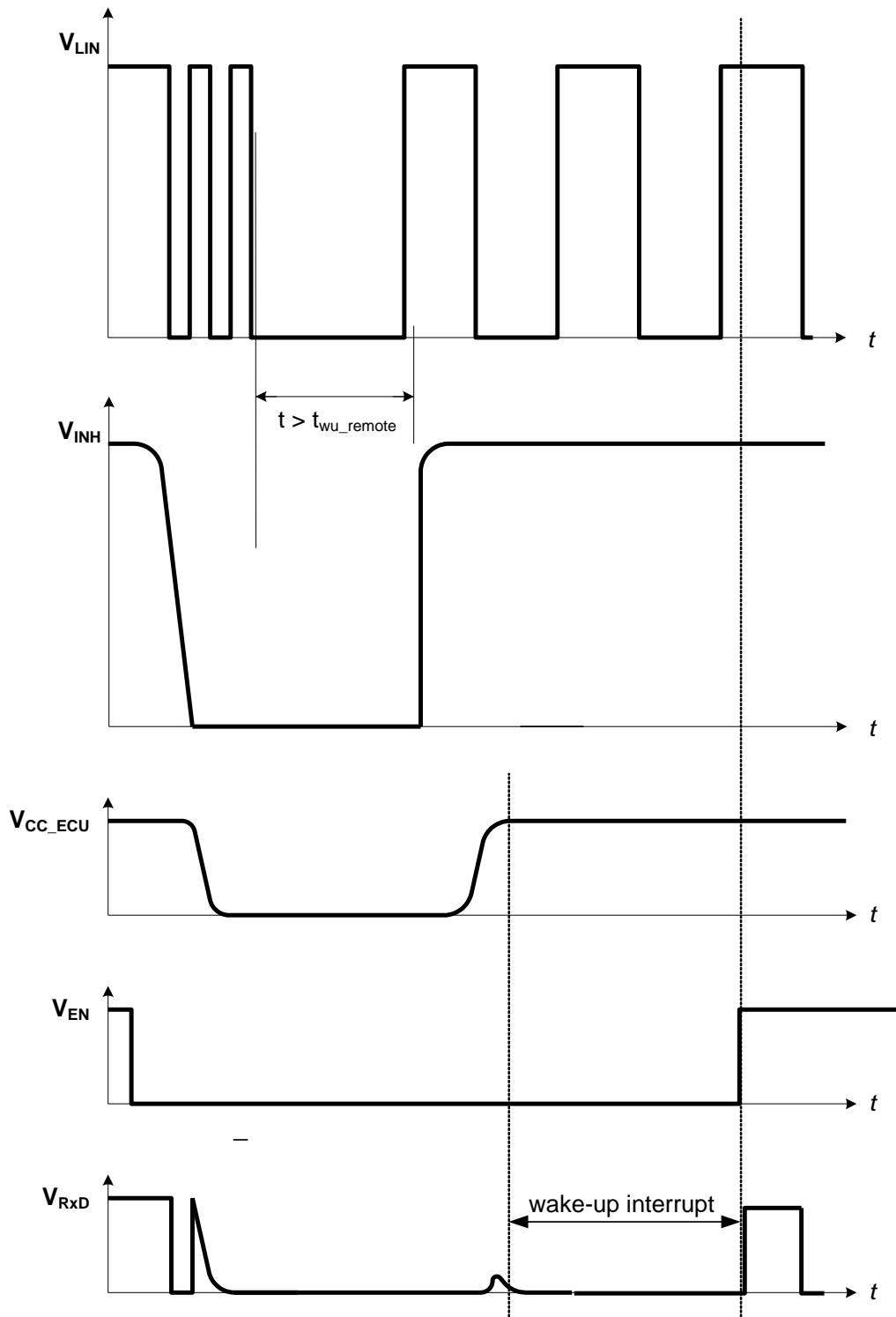
Figure 6: Remote wake-up behavior
