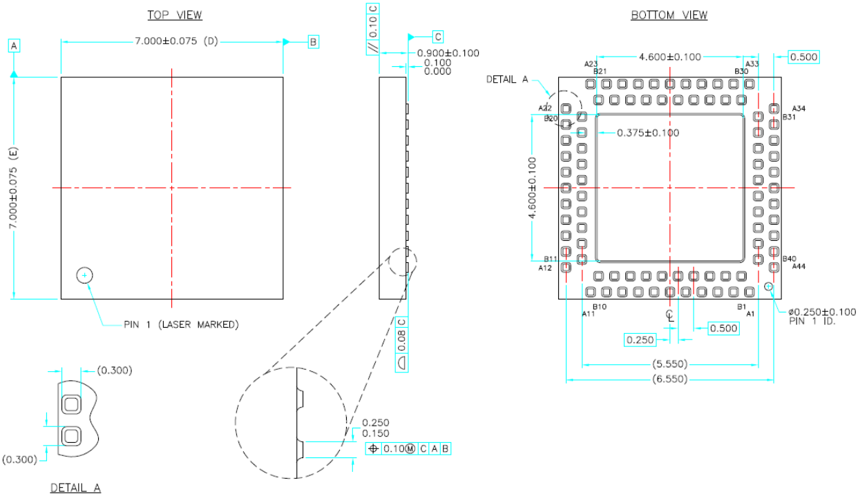
Figure 7 : Package dimensions
