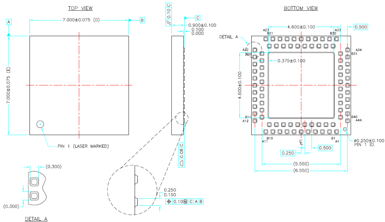
Figure 7 : Package dimensions
